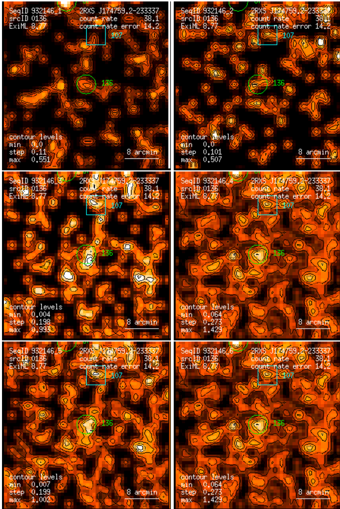
Figure 136: RASS 932146: detection 0136: band rate images, Gaussian filter: (1) PSPC channels 11 – 41, (2) 52 – 90, (3) 91 – 201, (4) 11 – 235, (5) 52 – 201, (6) 11 – 201. Broad band rates in counts/ks. Band rate contour levels in counts/ks/arcmin 2 .
