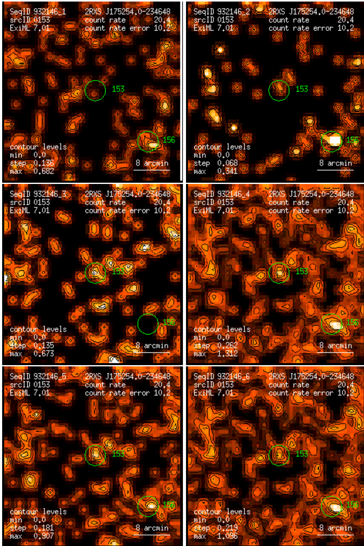
Figure 153: RASS 932146: detection 0153: band rate images, Gaussian filter: (1) PSPC channels 11 – 41, (2) 52 – 90, (3) 91 – 201, (4) 11 – 235, (5) 52 – 201, (6) 11 – 201. Broad band rates in counts/ks. Band rate contour levels in counts/ks/arcmin 2 .
