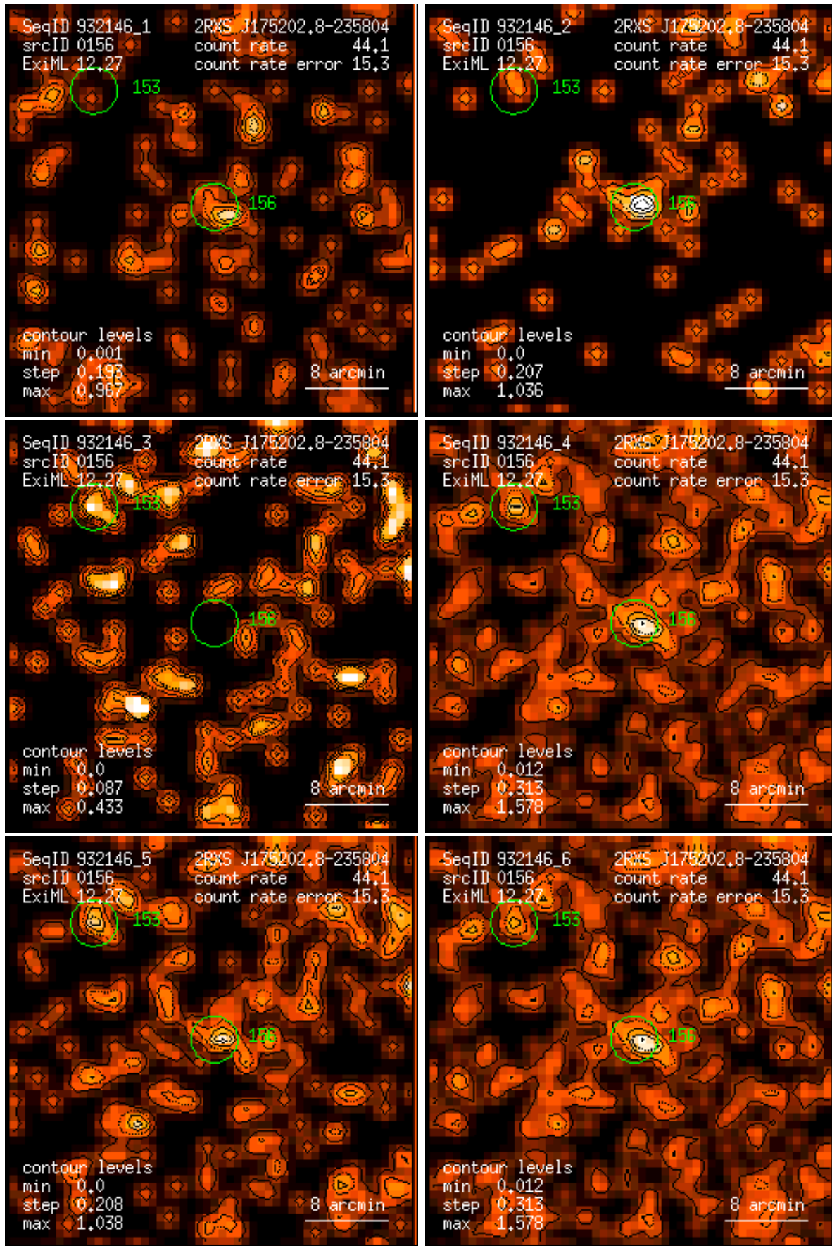
Figure 156: RASS 932146: detection 0156: band rate images, Gaussian filter: (1) PSPC channels 11 – 41, (2) 52 – 90, (3) 91 – 201, (4) 11 – 235, (5) 52 – 201, (6) 11 – 201. Broad band rates in counts/ks. Band rate contour levels in counts/ks/arcmin 2 .
