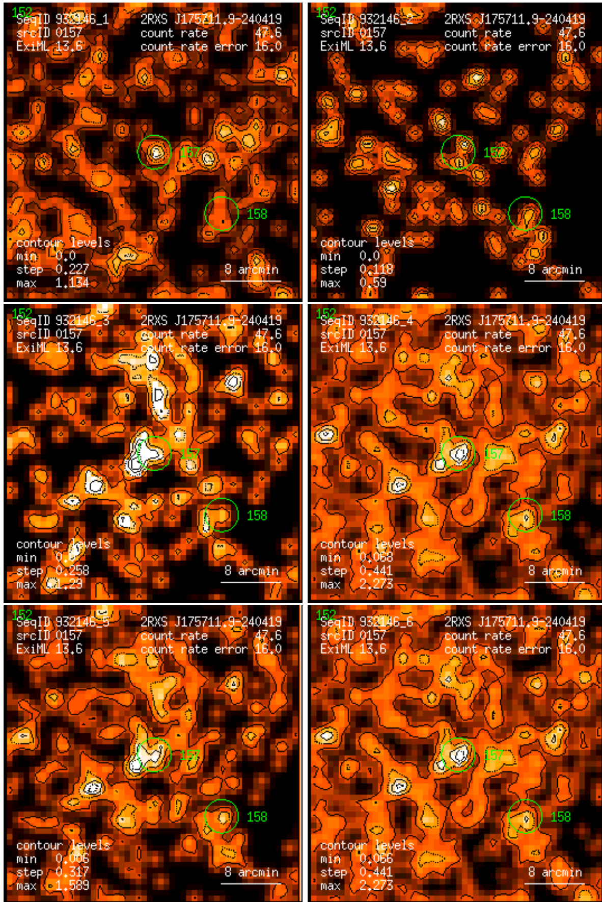
Figure 157: RASS 932146: detection 0157: band rate images, Gaussian filter: (1) PSPC channels 11 – 41, (2) 52 – 90, (3) 91 – 201, (4) 11 – 235, (5) 52 – 201, (6) 11 – 201. Broad band rates in counts/ks. Band rate contour levels in counts/ks/arcmin 2 .
