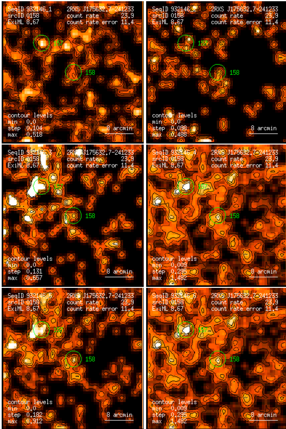
Figure 158: RASS 932146: detection 0158: band rate images, Gaussian filter: (1) PSPC channels 11 – 41, (2) 52 – 90, (3) 91 – 201, (4) 11 – 235, (5) 52 – 201, (6) 11 – 201. Broad band rates in counts/ks. Band rate contour levels in counts/ks/arcmin 2 .
