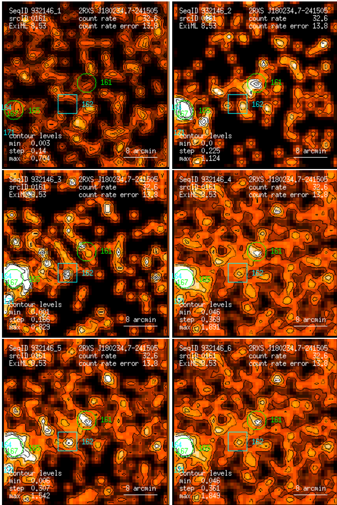
Figure 161: RASS 932146: detection 0161: band rate images, Gaussian filter: (1) PSPC channels 11 – 41, (2) 52 – 90, (3) 91 – 201, (4) 11 – 235, (5) 52 – 201, (6) 11 – 201. Broad band rates in counts/ks. Band rate contour levels in counts/ks/arcmin 2 .
