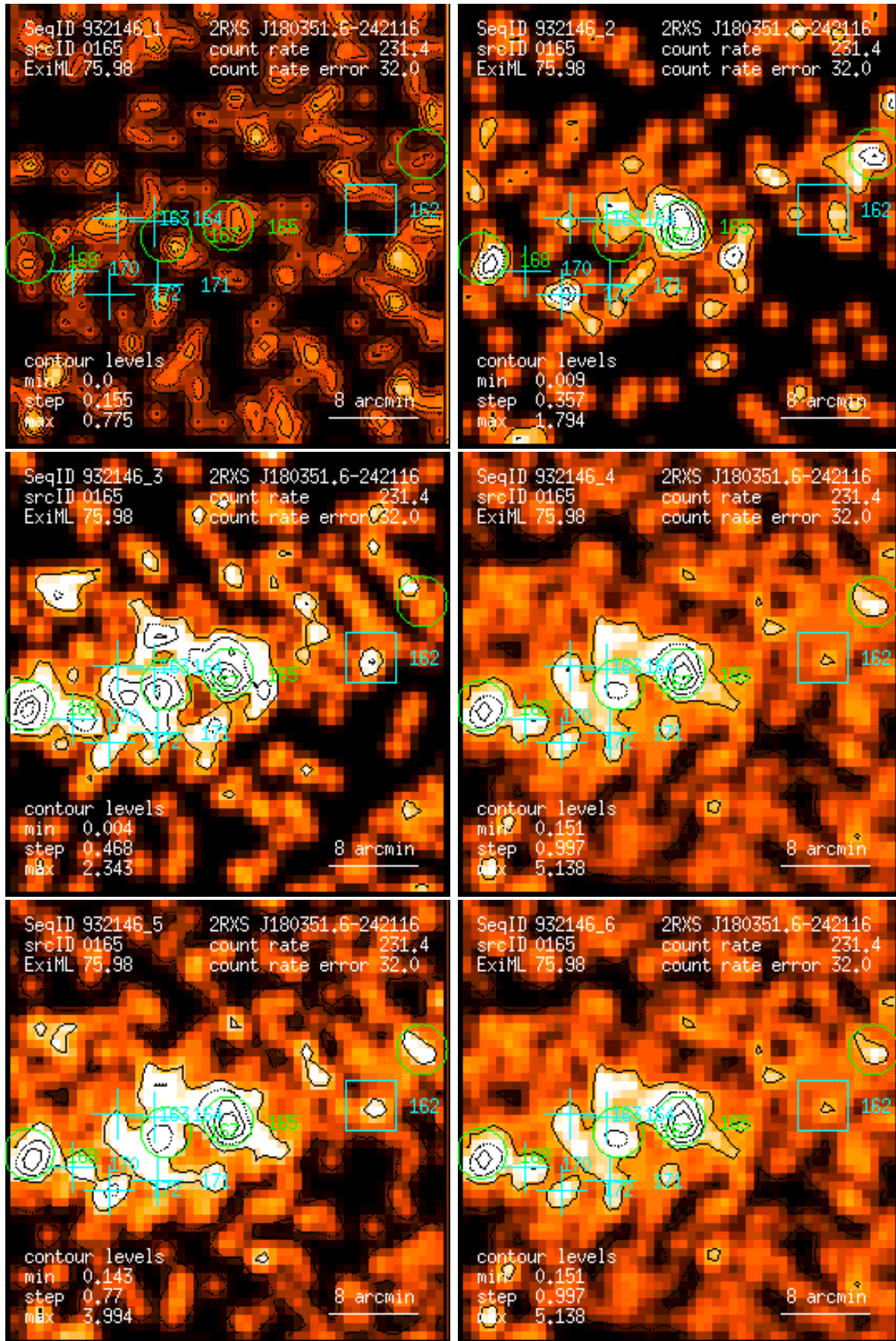
Figure 165: RASS 932146: detection 0165: band rate images, Gaussian filter: (1) PSPC channels 11 – 41, (2) 52 – 90, (3) 91 – 201, (4) 11 – 235, (5) 52 – 201, (6) 11 – 201. Broad band rates in counts/ks. Band rate contour levels in counts/ks/arcmin 2 .
