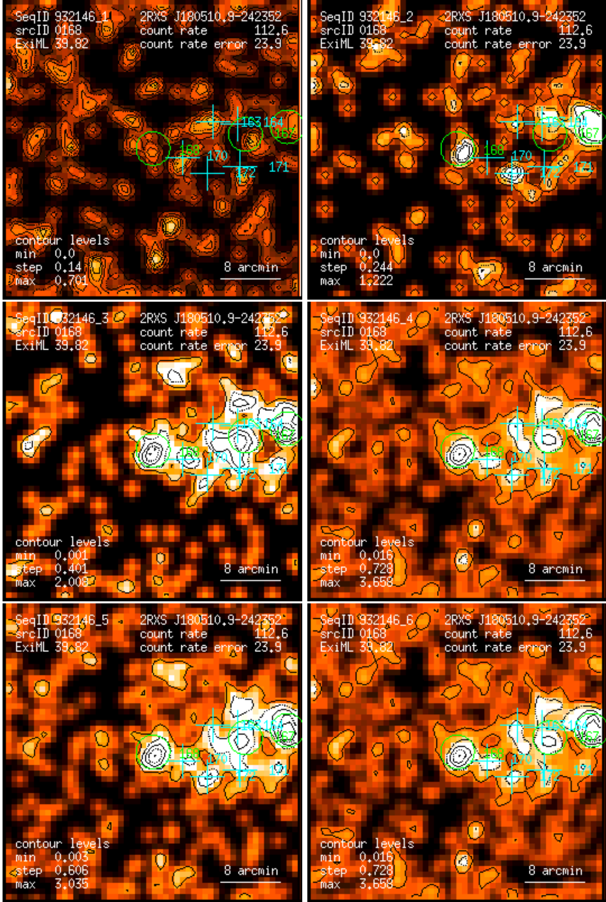
Figure 168: RASS 932146: detection 0168: band rate images, Gaussian filter: (1) PSPC channels 11 – 41, (2) 52 – 90, (3) 91 – 201, (4) 11 – 235, (5) 52 – 201, (6) 11 – 201. Broad band rates in counts/ks. Band rate contour levels in counts/ks/arcmin 2 .
