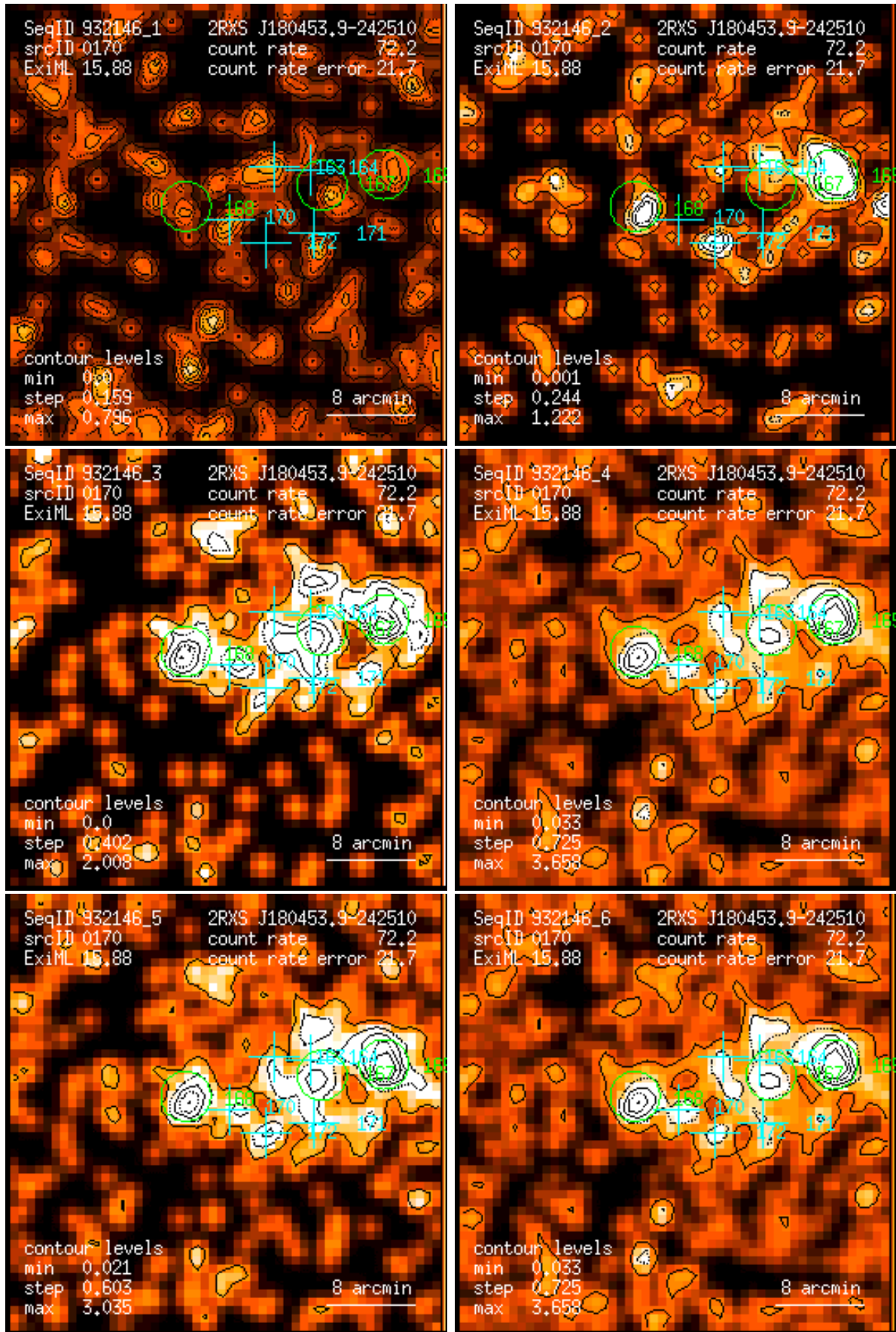
Figure 170: RASS 932146: detection 0170: band rate images, Gaussian filter: (1) PSPC channels 11 – 41, (2) 52 – 90, (3) 91 – 201, (4) 11 – 235, (5) 52 – 201, (6) 11 – 201. Broad band rates in counts/ks. Band rate contour levels in counts/ks/arcmin 2 .
