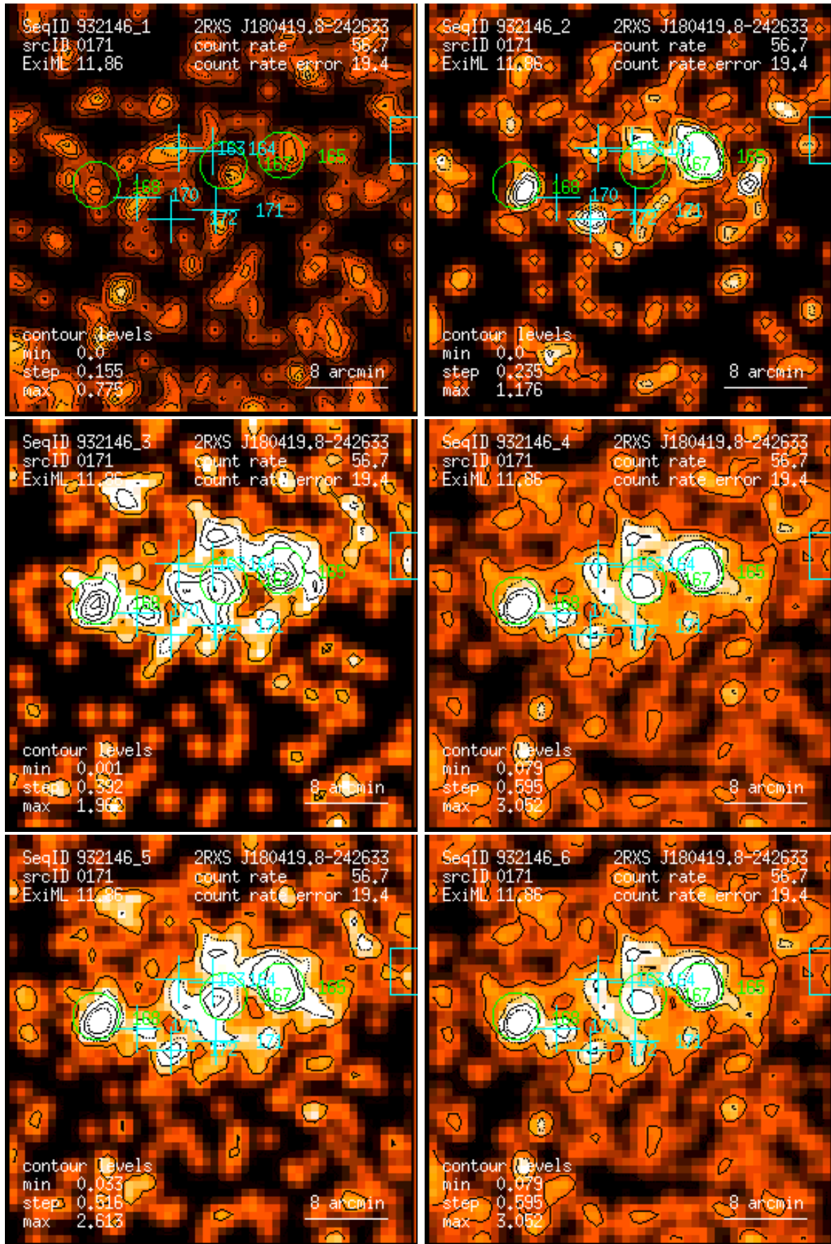
Figure 171: RASS 932146: detection 0171: band rate images, Gaussian filter: (1) PSPC channels 11 – 41, (2) 52 – 90, (3) 91 – 201, (4) 11 – 235, (5) 52 – 201, (6) 11 – 201. Broad band rates in counts/ks. Band rate contour levels in counts/ks/arcmin 2 .
