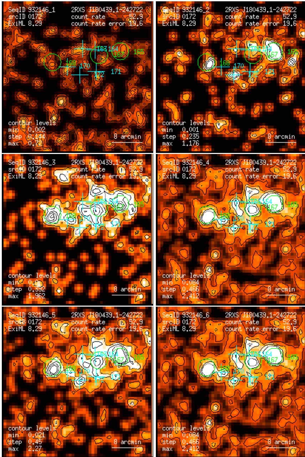
Figure 172: RASS 932146: detection 0172: band rate images, Gaussian filter: (1) PSPC channels 11 – 41, (2) 52 – 90, (3) 91 – 201, (4) 11 – 235, (5) 52 – 201, (6) 11 – 201. Broad band rates in counts/ks. Band rate contour levels in counts/ks/arcmin 2 .
