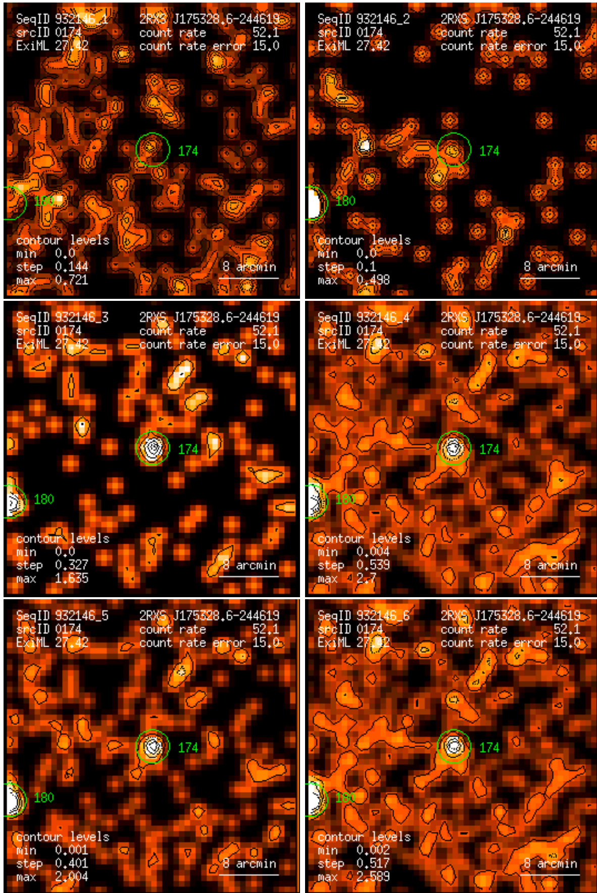
Figure 174: RASS 932146: detection 0174: band rate images, Gaussian filter: (1) PSPC channels 11 – 41, (2) 52 – 90, (3) 91 – 201, (4) 11 – 235, (5) 52 – 201, (6) 11 – 201. Broad band rates in counts/ks. Band rate contour levels in counts/ks/arcmin 2 .
