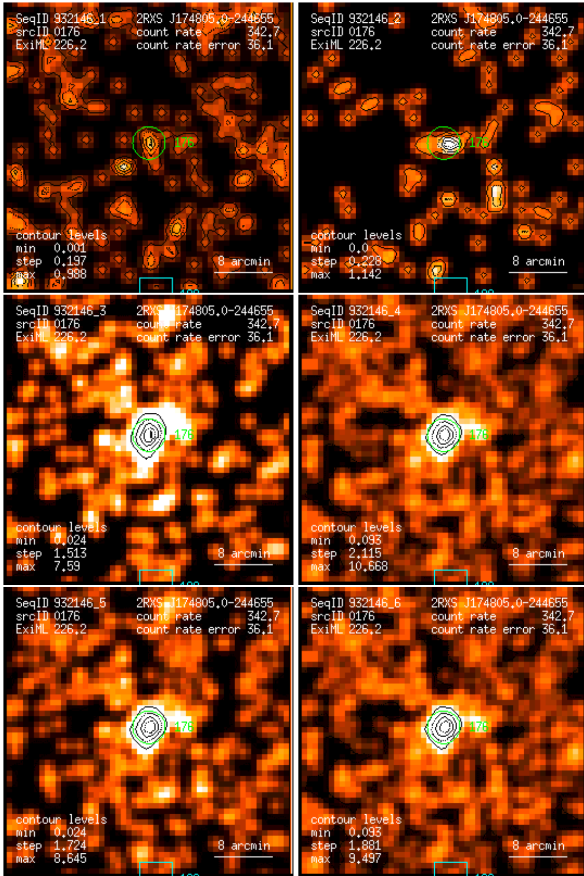
Figure 176: RASS 932146: detection 0176: band rate images, Gaussian filter: (1) PSPC channels 11 – 41, (2) 52 – 90, (3) 91 – 201, (4) 11 – 235, (5) 52 – 201, (6) 11 – 201. Broad band rates in counts/ks. Band rate contour levels in counts/ks/arcmin 2 .
