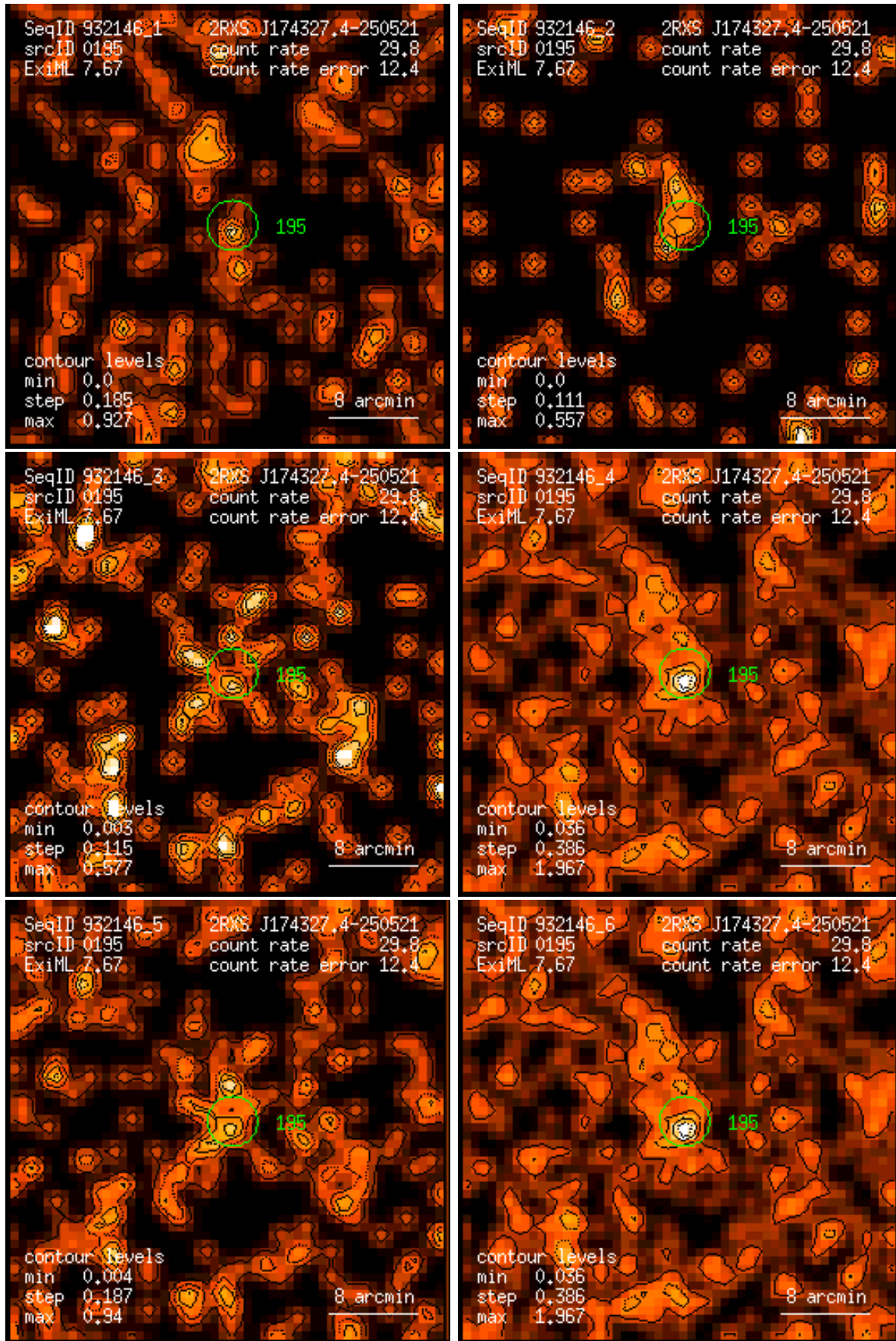
Figure 195: RASS 932146: detection 0195: band rate images, Gaussian filter: (1) PSPC channels 11 – 41, (2) 52 – 90, (3) 91 – 201, (4) 11 – 235, (5) 52 – 201, (6) 11 – 201. Broad band rates in counts/ks. Band rate contour levels in counts/ks/arcmin 2 .
