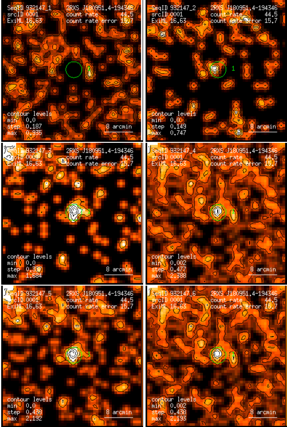
Figure 1: RASS 932147: detection 0001: band rate images, Gaussian filter: (1) PSPC channels 11 – 41, (2) 52 – 90, (3) 91 – 201, (4) 11 – 235, (5) 52 – 201, (6) 11 – 201. Broad band rates in counts/ks. Band rate contour levels in counts/ks/arcmin 2 .
