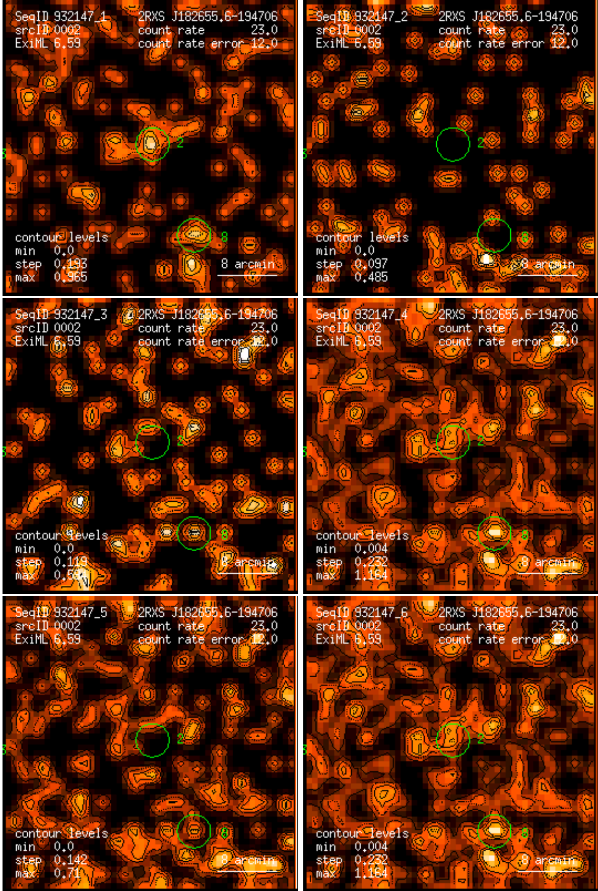
Figure 2: RASS 932147: detection 0002: band rate images, Gaussian filter: (1) PSPC channels 11 – 41, (2) 52 – 90, (3) 91 – 201, (4) 11 – 235, (5) 52 – 201, (6) 11 – 201. Broad band rates in counts/ks. Band rate contour levels in counts/ks/arcmin 2 .
