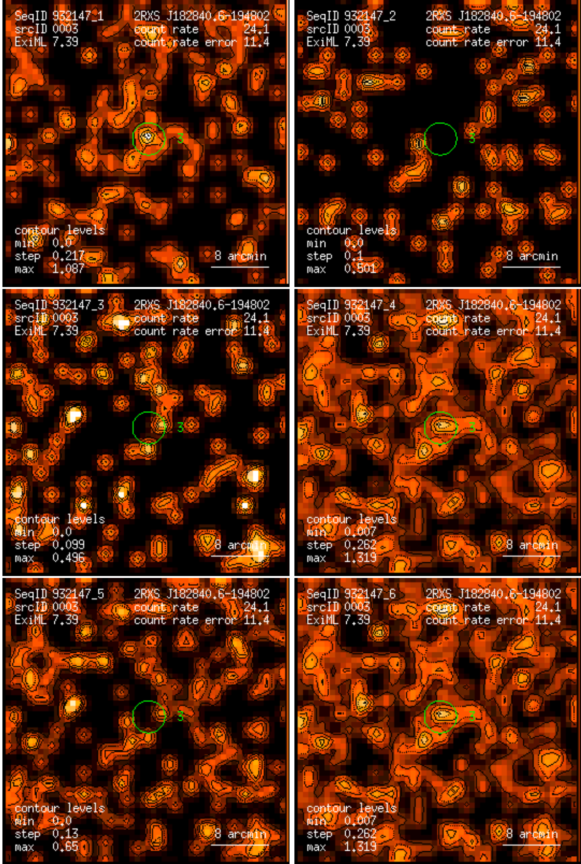
Figure 3: RASS 932147: detection 0003: band rate images, Gaussian filter: (1) PSPC channels 11 – 41, (2) 52 – 90, (3) 91 – 201, (4) 11 – 235, (5) 52 – 201, (6) 11 – 201. Broad band rates in counts/ks. Band rate contour levels in counts/ks/arcmin 2 .
