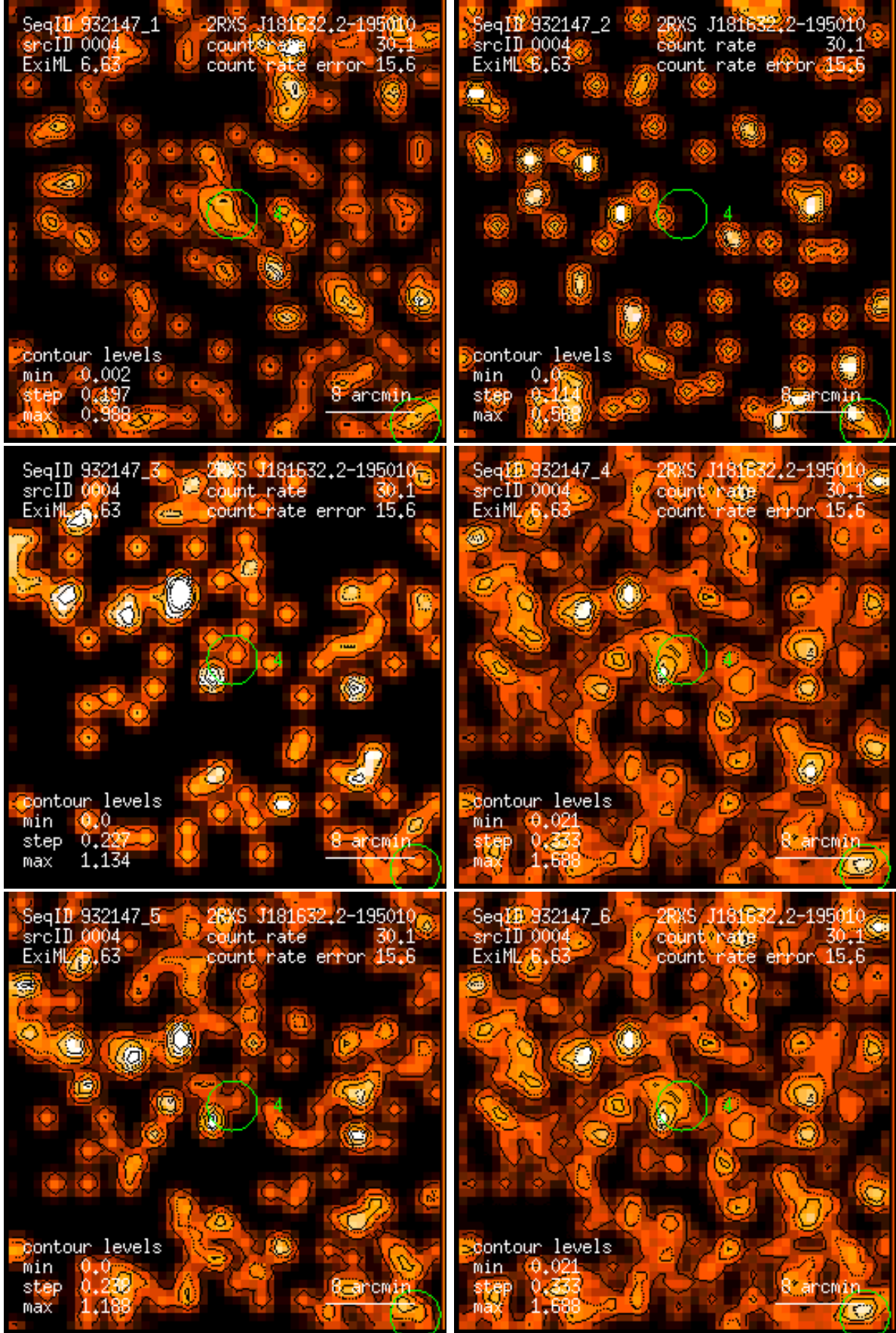
Figure 4: RASS 932147: detection 0004: band rate images, Gaussian filter: (1) PSPC channels 11 – 41, (2) 52 – 90, (3) 91 – 201, (4) 11 – 235, (5) 52 – 201, (6) 11 – 201. Broad band rates in counts/ks. Band rate contour levels in counts/ks/arcmin 2 .
