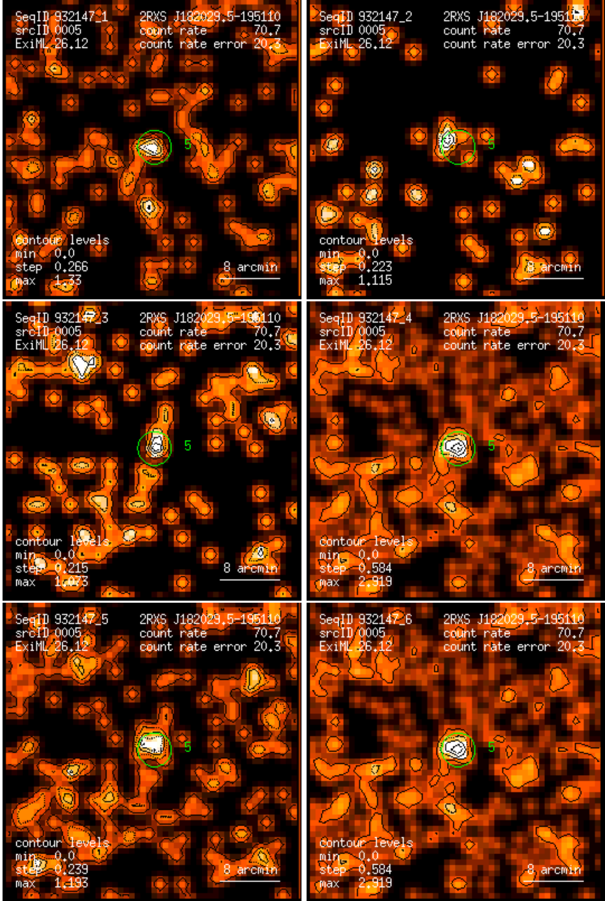
Figure 5: RASS 932147: detection 0005: band rate images, Gaussian filter: (1) PSPC channels 11 – 41, (2) 52 – 90, (3) 91 – 201, (4) 11 – 235, (5) 52 – 201, (6) 11 – 201. Broad band rates in counts/ks. Band rate contour levels in counts/ks/arcmin 2 .
