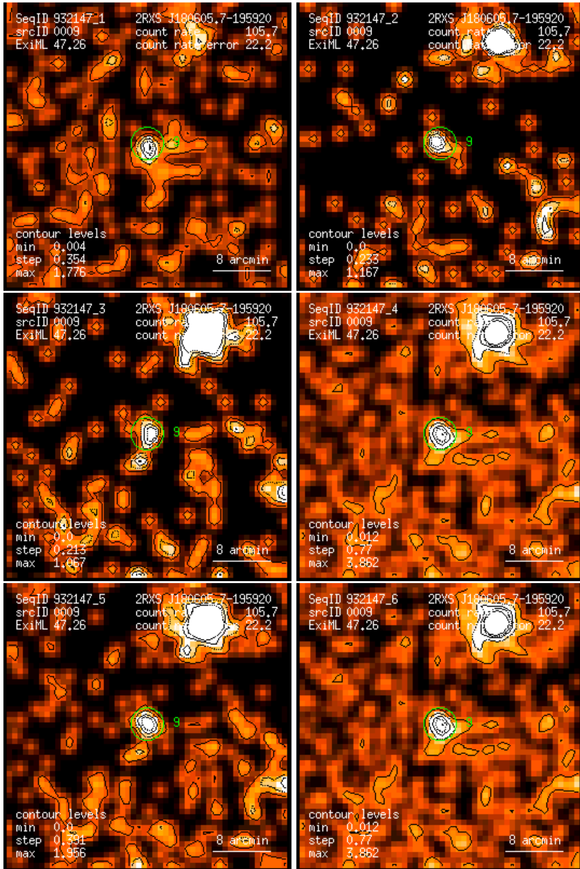
Figure 9: RASS 932147: detection 0009: band rate images, Gaussian filter: (1) PSPC channels 11 – 41, (2) 52 – 90, (3) 91 – 201, (4) 11 – 235, (5) 52 – 201, (6) 11 – 201. Broad band rates in counts/ks. Band rate contour levels in counts/ks/arcmin 2 .
