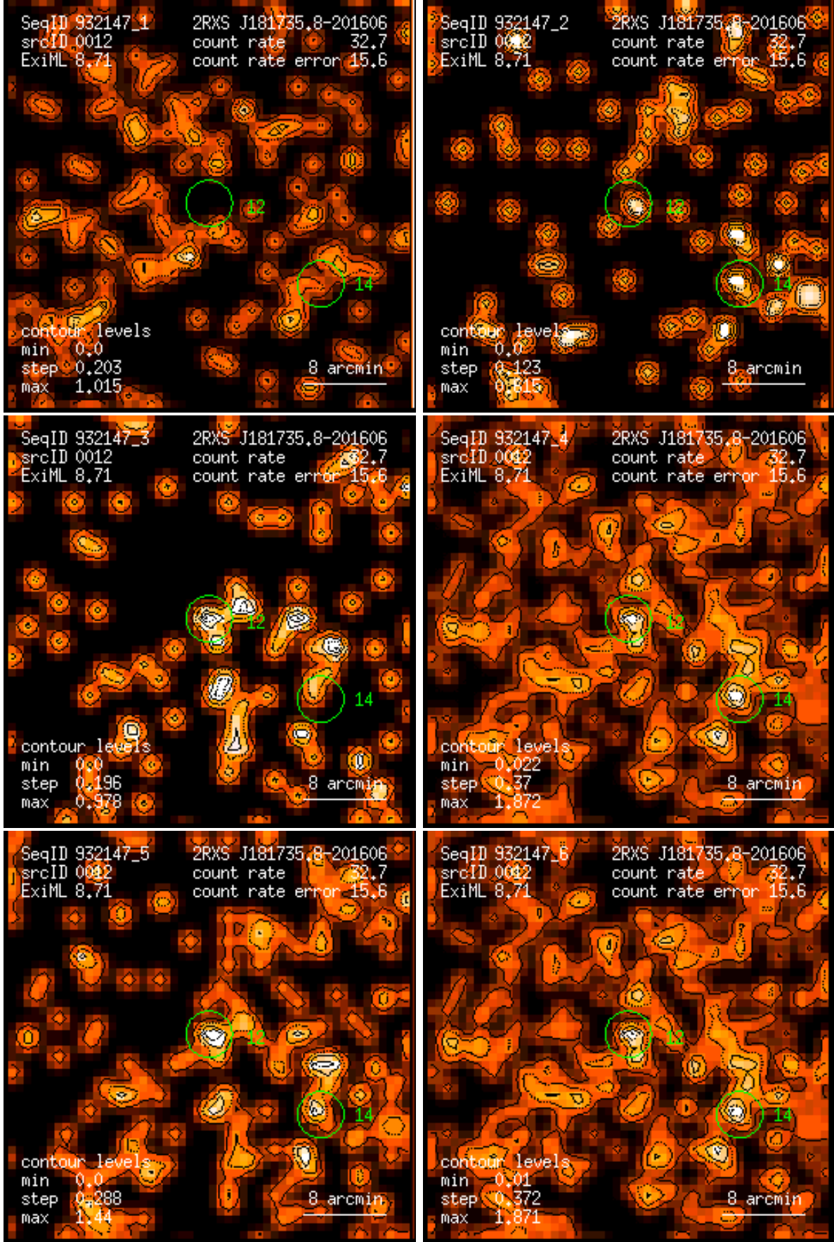
Figure 12: RASS 932147: detection 0012: band rate images, Gaussian filter: (1) PSPC channels 11 – 41, (2) 52 – 90, (3) 91 – 201, (4) 11 – 235, (5) 52 – 201, (6) 11 – 201. Broad band rates in counts/ks. Band rate contour levels in counts/ks/arcmin 2 .
