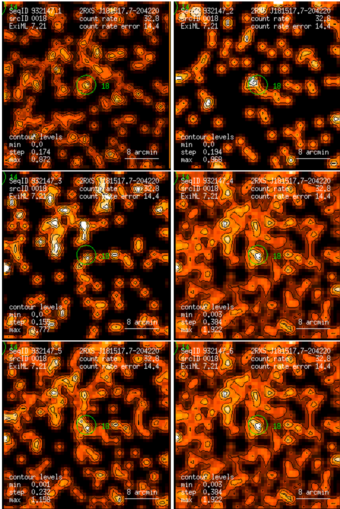
Figure 18: RASS 932147: detection 0018: band rate images, Gaussian filter: (1) PSPC channels 11 – 41, (2) 52 – 90, (3) 91 – 201, (4) 11 – 235, (5) 52 – 201, (6) 11 – 201. Broad band rates in counts/ks. Band rate contour levels in counts/ks/arcmin 2 .
