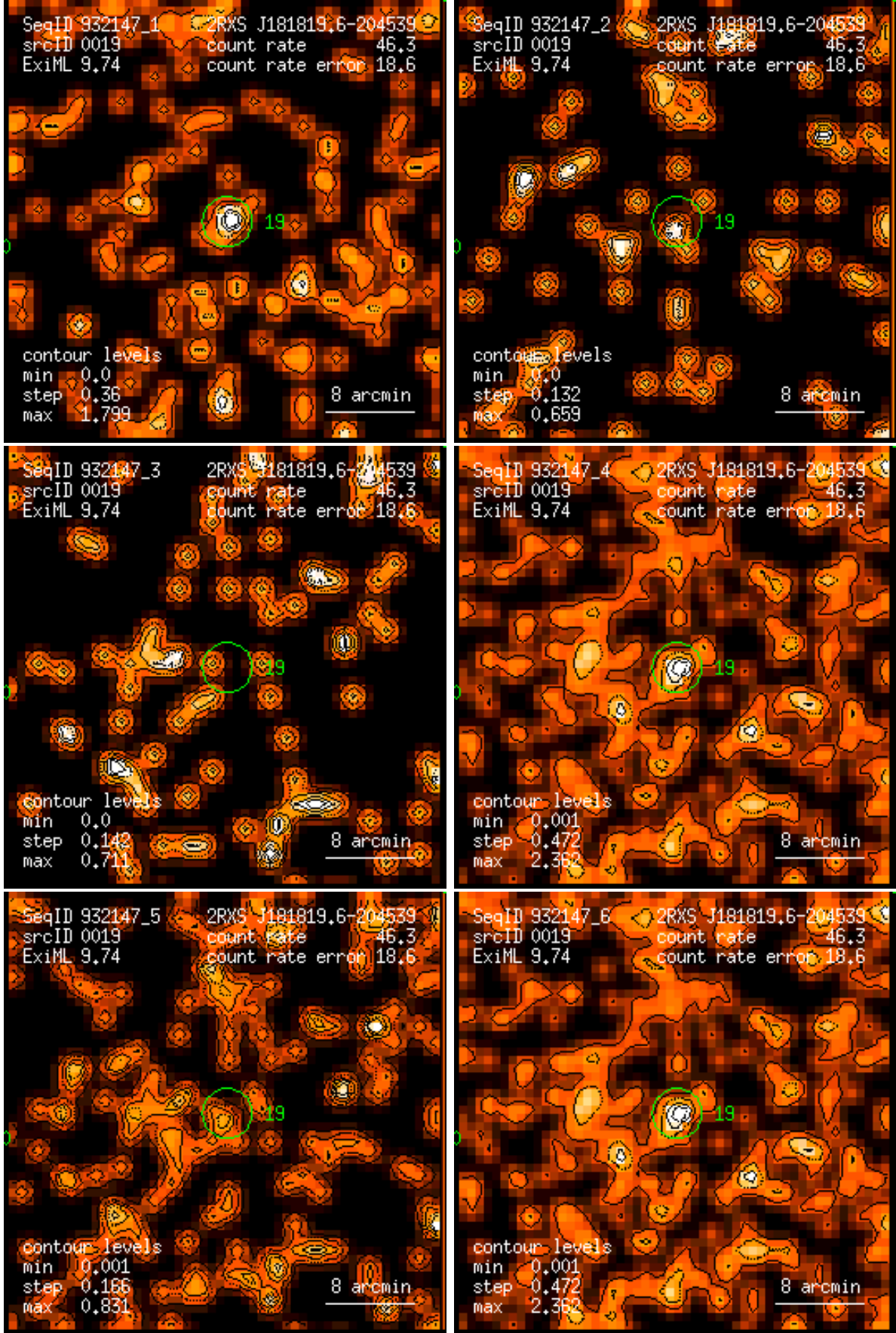
Figure 19: RASS 932147: detection 0019: band rate images, Gaussian filter: (1) PSPC channels 11 – 41, (2) 52 – 90, (3) 91 – 201, (4) 11 – 235, (5) 52 – 201, (6) 11 – 201. Broad band rates in counts/ks. Band rate contour levels in counts/ks/arcmin 2 .
