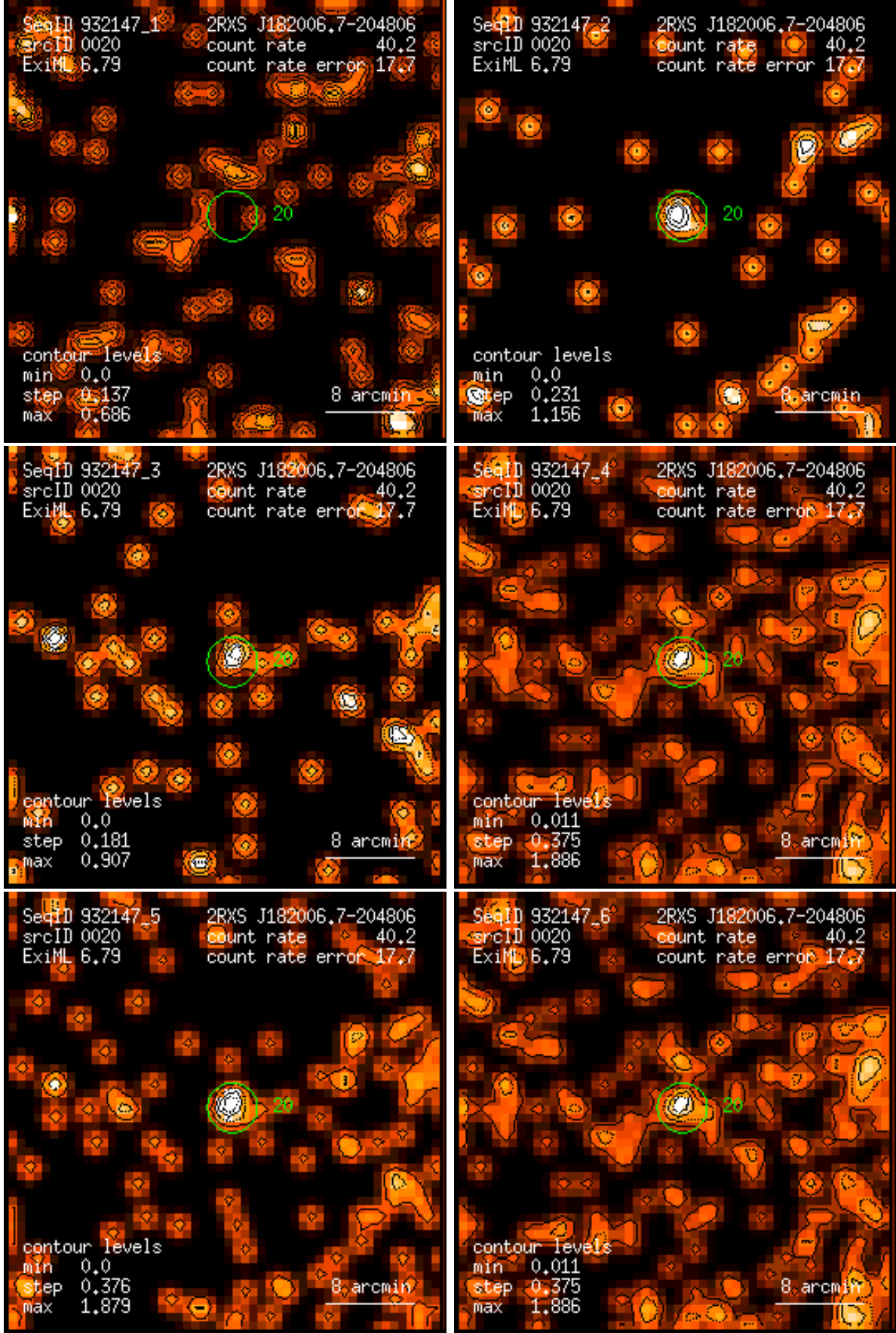
Figure 20: RASS 932147: detection 0020: band rate images, Gaussian filter: (1) PSPC channels 11 – 41, (2) 52 – 90, (3) 91 – 201, (4) 11 – 235, (5) 52 – 201, (6) 11 – 201. Broad band rates in counts/ks. Band rate contour levels in counts/ks/arcmin 2 .
