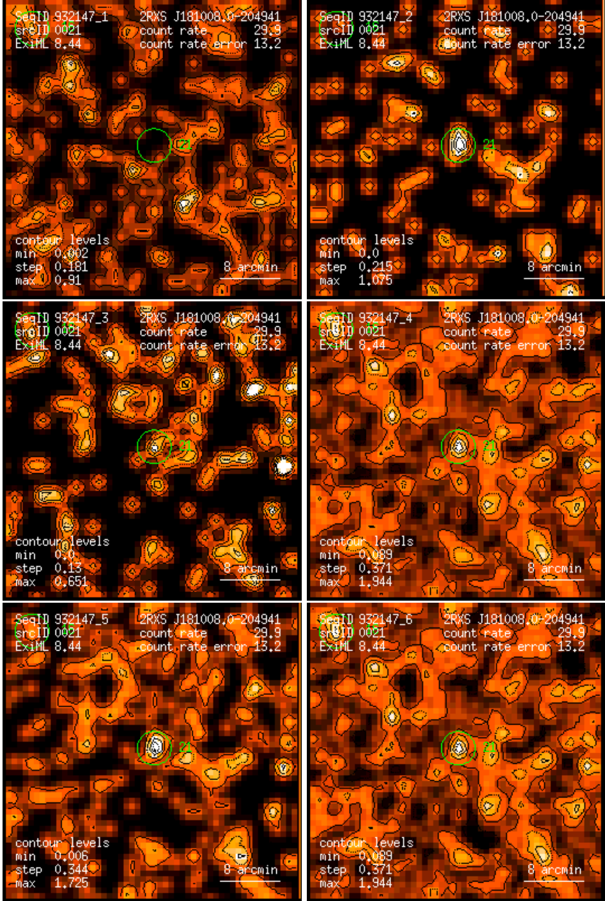
Figure 21: RASS 932147: detection 0021: band rate images, Gaussian filter: (1) PSPC channels 11 – 41, (2) 52 – 90, (3) 91 – 201, (4) 11 – 235, (5) 52 – 201, (6) 11 – 201. Broad band rates in counts/ks. Band rate contour levels in counts/ks/arcmin 2 .
