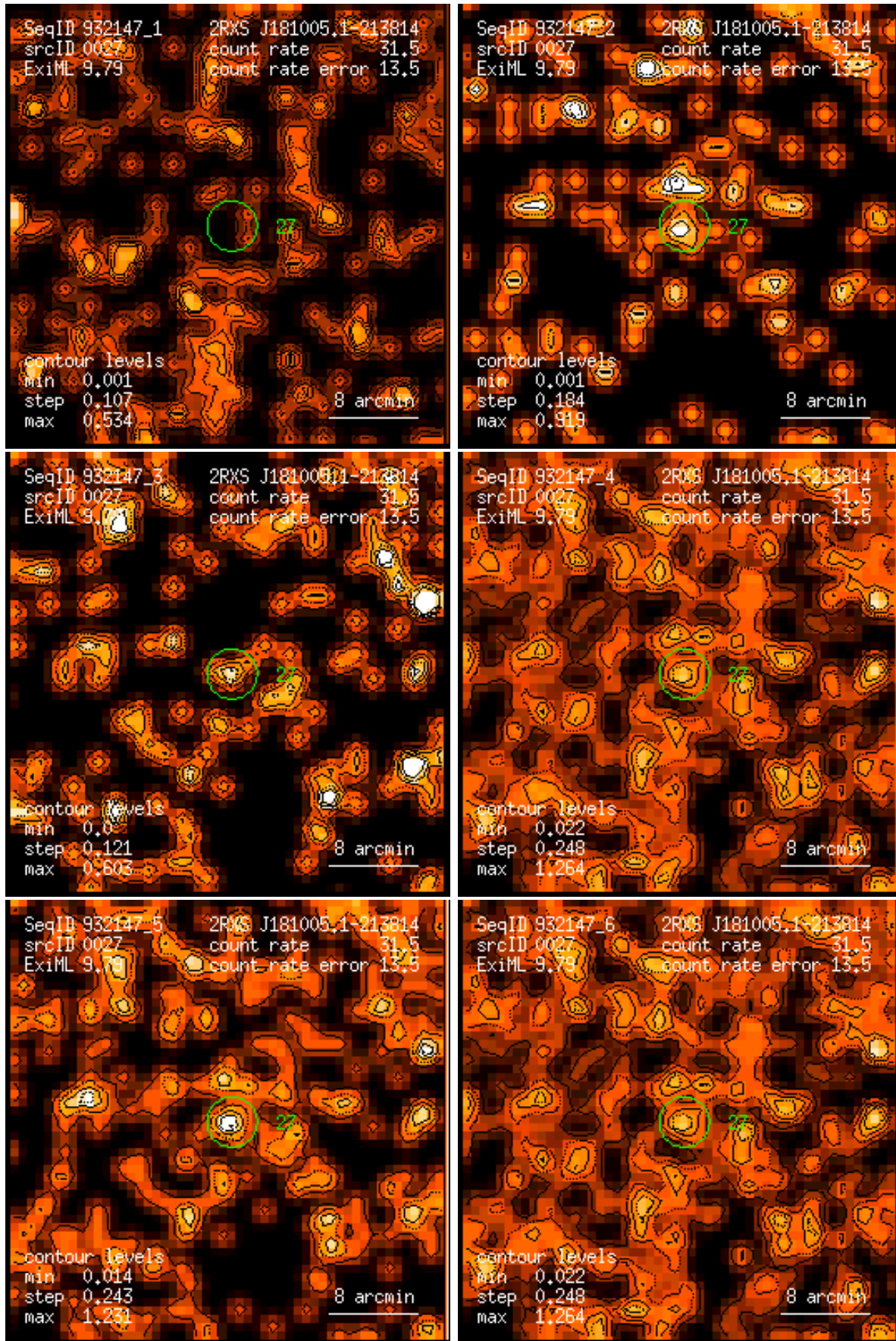
Figure 27: RASS 932147: detection 0027: band rate images, Gaussian filter: (1) PSPC channels 11 – 41, (2) 52 – 90, (3) 91 – 201, (4) 11 – 235, (5) 52 – 201, (6) 11 – 201. Broad band rates in counts/ks. Band rate contour levels in counts/ks/arcmin 2 .
