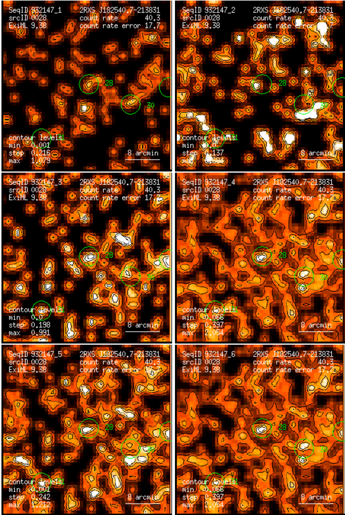
Figure 28: RASS 932147: detection 0028: band rate images, Gaussian filter: (1) PSPC channels 11 – 41, (2) 52 – 90, (3) 91 – 201, (4) 11 – 235, (5) 52 – 201, (6) 11 – 201. Broad band rates in counts/ks. Band rate contour levels in counts/ks/arcmin 2 .
