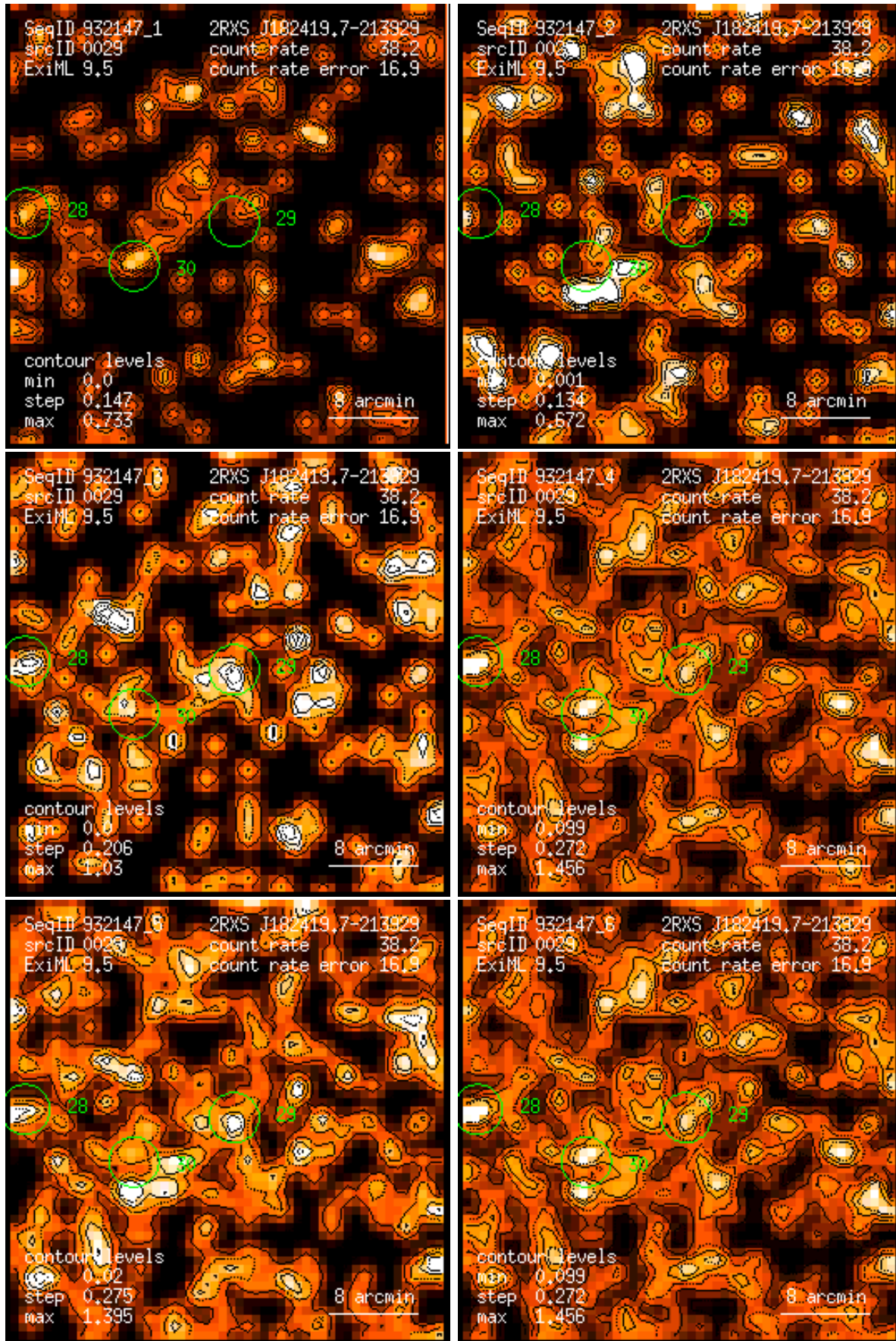
Figure 29: RASS 932147: detection 0029: band rate images, Gaussian filter: (1) PSPC channels 11 – 41, (2) 52 – 90, (3) 91 – 201, (4) 11 – 235, (5) 52 – 201, (6) 11 – 201. Broad band rates in counts/ks. Band rate contour levels in counts/ks/arcmin 2 .
