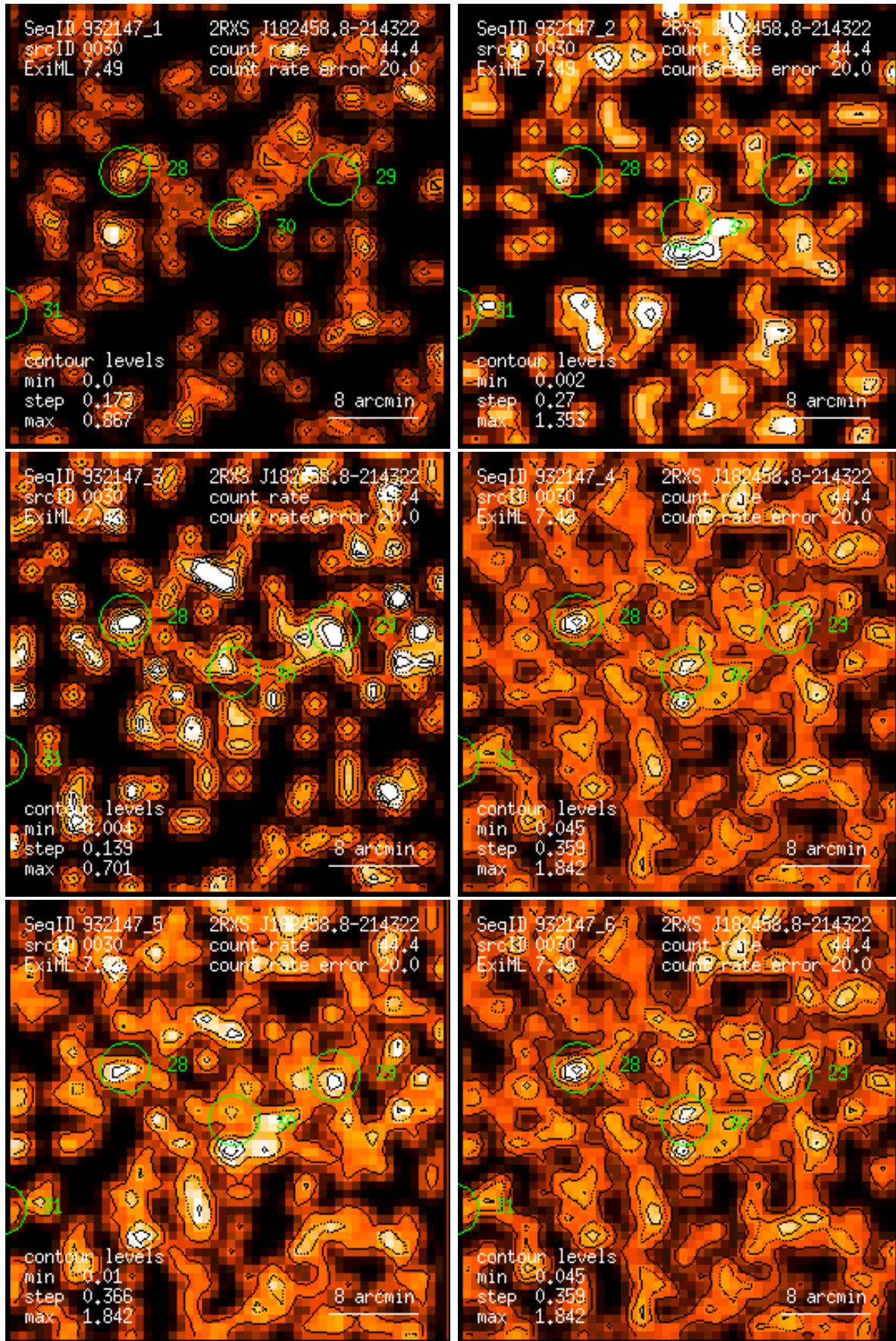
Figure 30: RASS 932147: detection 0030: band rate images, Gaussian filter: (1) PSPC channels 11 – 41, (2) 52 – 90, (3) 91 – 201, (4) 11 – 235, (5) 52 – 201, (6) 11 – 201. Broad band rates in counts/ks. Band rate contour levels in counts/ks/arcmin 2 .
