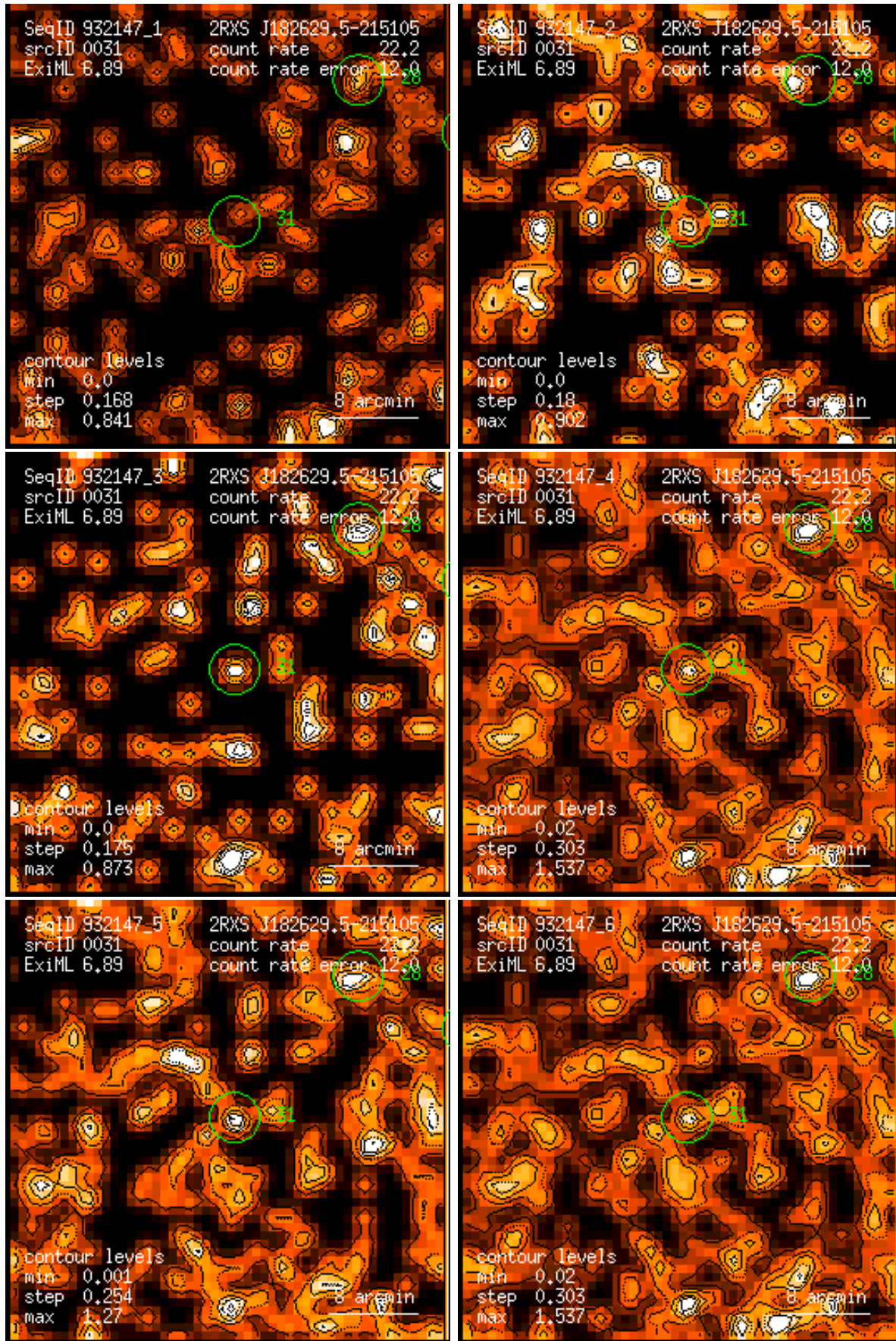
Figure 31: RASS 932147: detection 0031: band rate images, Gaussian filter: (1) PSPC channels 11 – 41, (2) 52 – 90, (3) 91 – 201, (4) 11 – 235, (5) 52 – 201, (6) 11 – 201. Broad band rates in counts/ks. Band rate contour levels in counts/ks/arcmin 2 .
