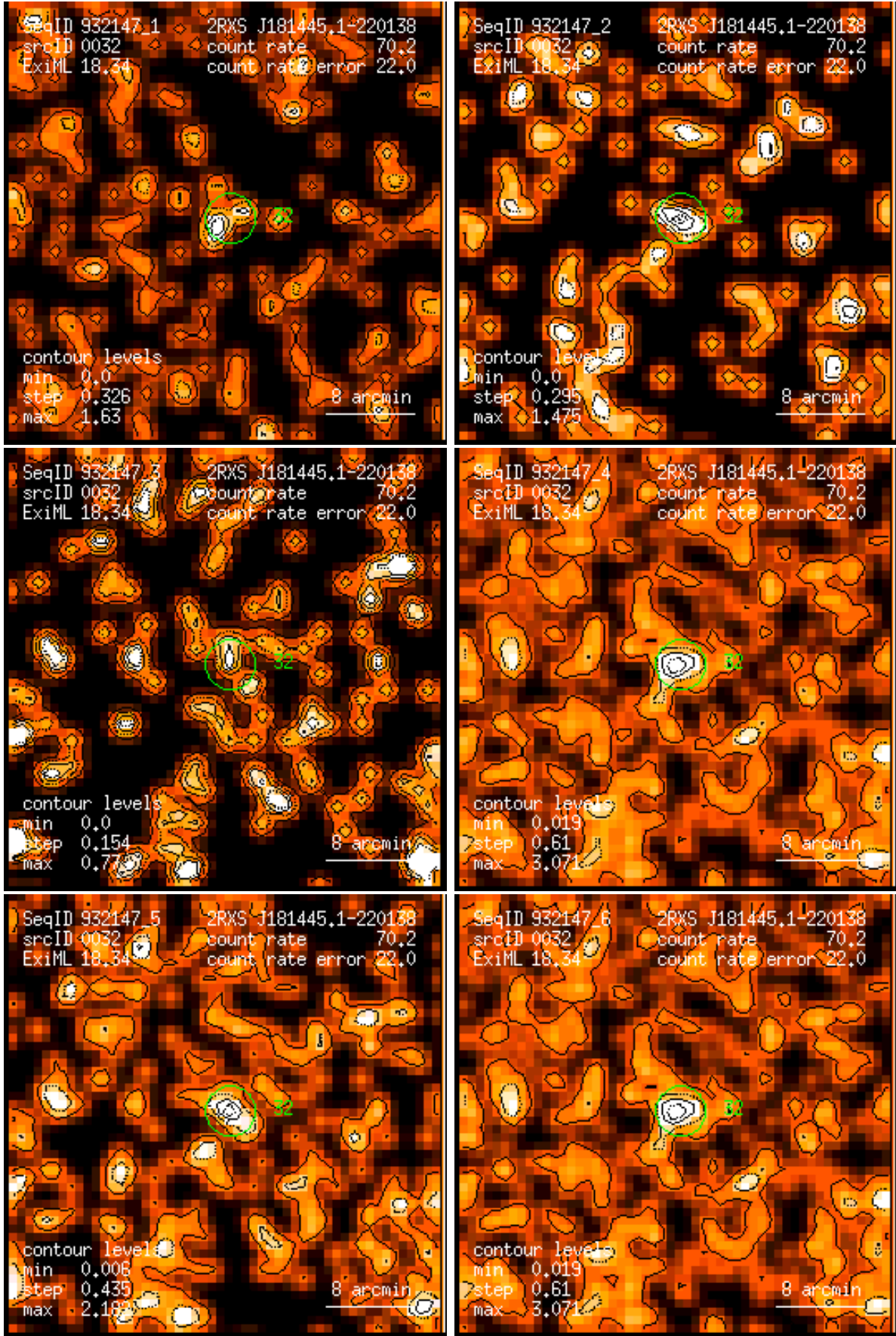
Figure 32: RASS 932147: detection 0032: band rate images, Gaussian filter: (1) PSPC channels 11 – 41, (2) 52 – 90, (3) 91 – 201, (4) 11 – 235, (5) 52 – 201, (6) 11 – 201. Broad band rates in counts/ks. Band rate contour levels in counts/ks/arcmin 2 .
