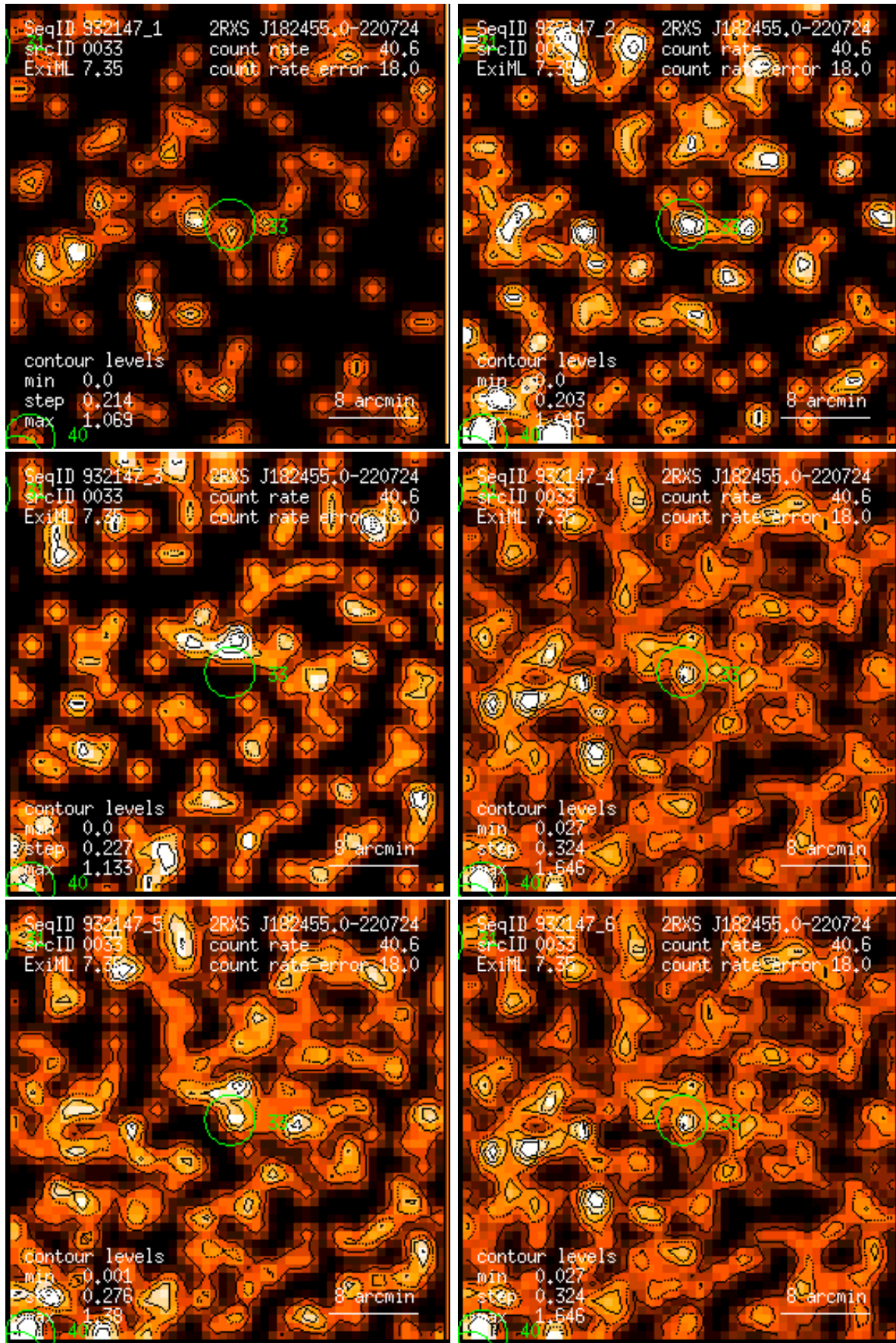
Figure 33: RASS 932147: detection 0033: band rate images, Gaussian filter: (1) PSPC channels 11 – 41, (2) 52 – 90, (3) 91 – 201, (4) 11 – 235, (5) 52 – 201, (6) 11 – 201. Broad band rates in counts/ks. Band rate contour levels in counts/ks/arcmin 2 .
