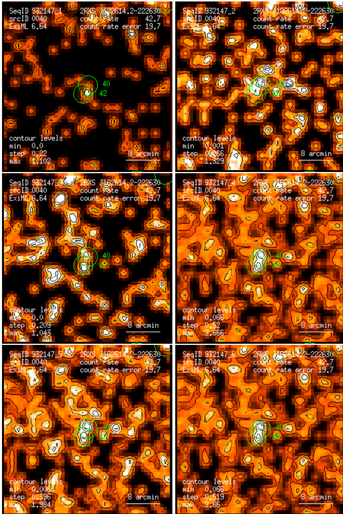
Figure 40: RASS 932147: detection 0040: band rate images, Gaussian filter: (1) PSPC channels 11 – 41, (2) 52 – 90, (3) 91 – 201, (4) 11 – 235, (5) 52 – 201, (6) 11 – 201. Broad band rates in counts/ks. Band rate contour levels in counts/ks/arcmin 2 .
