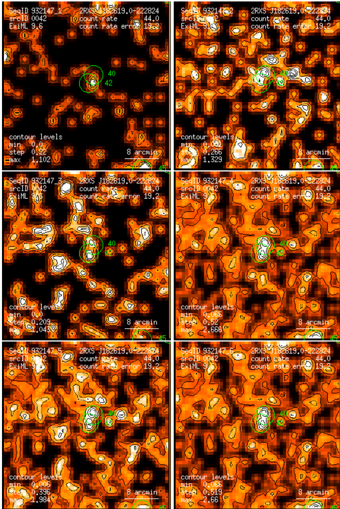
Figure 42: RASS 932147: detection 0042: band rate images, Gaussian filter: (1) PSPC channels 11 – 41, (2) 52 – 90, (3) 91 – 201, (4) 11 – 235, (5) 52 – 201, (6) 11 – 201. Broad band rates in counts/ks. Band rate contour levels in counts/ks/arcmin 2 .
