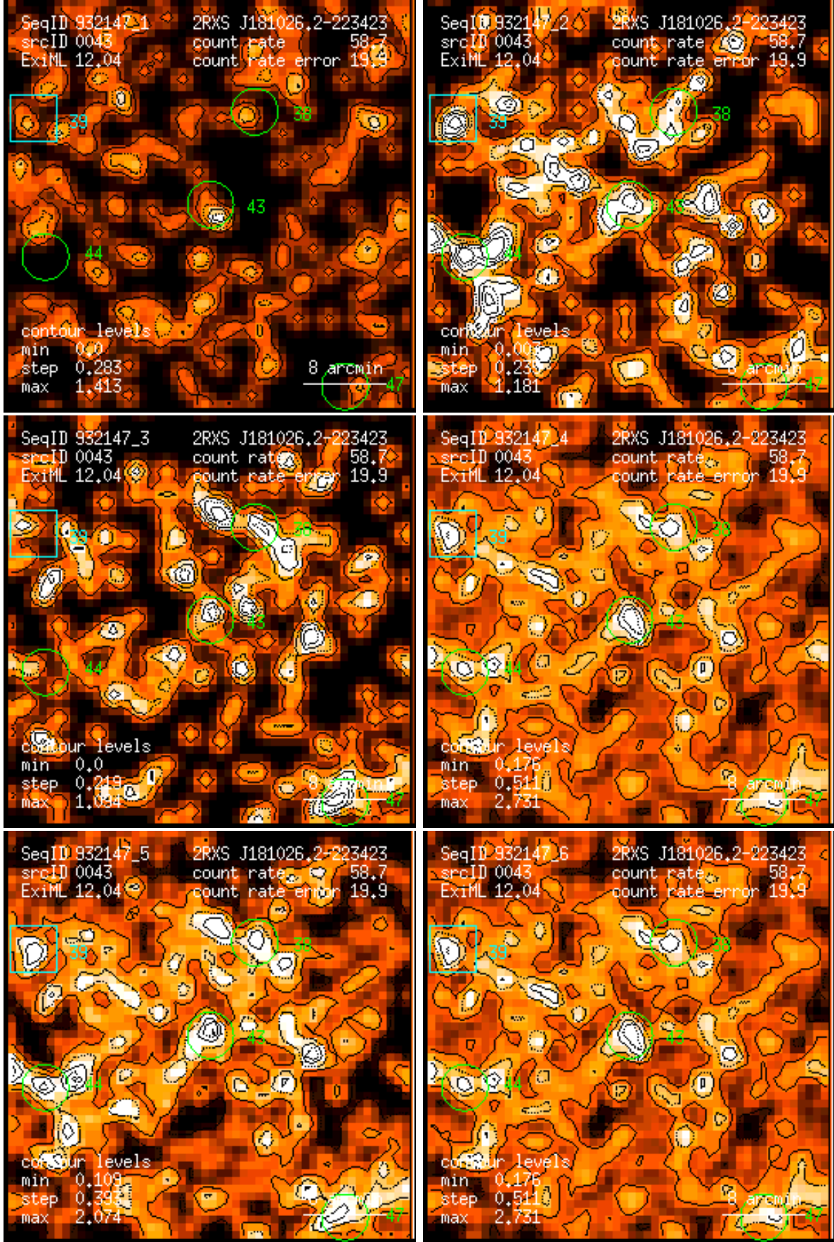
Figure 43: RASS 932147: detection 0043: band rate images, Gaussian filter: (1) PSPC channels 11 – 41, (2) 52 – 90, (3) 91 – 201, (4) 11 – 235, (5) 52 – 201, (6) 11 – 201. Broad band rates in counts/ks. Band rate contour levels in counts/ks/arcmin 2 .
