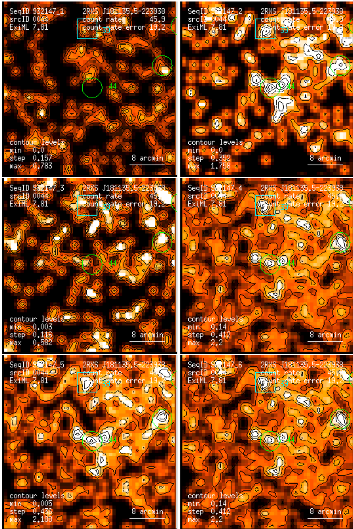
Figure 44: RASS 932147: detection 0044: band rate images, Gaussian filter: (1) PSPC channels 11 – 41, (2) 52 – 90, (3) 91 – 201, (4) 11 – 235, (5) 52 – 201, (6) 11 – 201. Broad band rates in counts/ks. Band rate contour levels in counts/ks/arcmin 2 .
