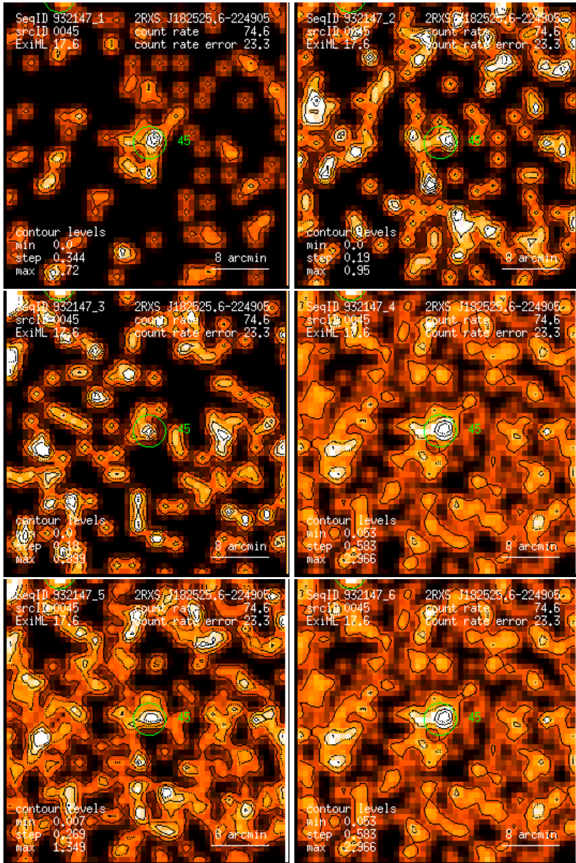
Figure 45: RASS 932147: detection 0045: band rate images, Gaussian filter: (1) PSPC channels 11 – 41, (2) 52 – 90, (3) 91 – 201, (4) 11 – 235, (5) 52 – 201, (6) 11 – 201. Broad band rates in counts/ks. Band rate contour levels in counts/ks/arcmin 2 .
