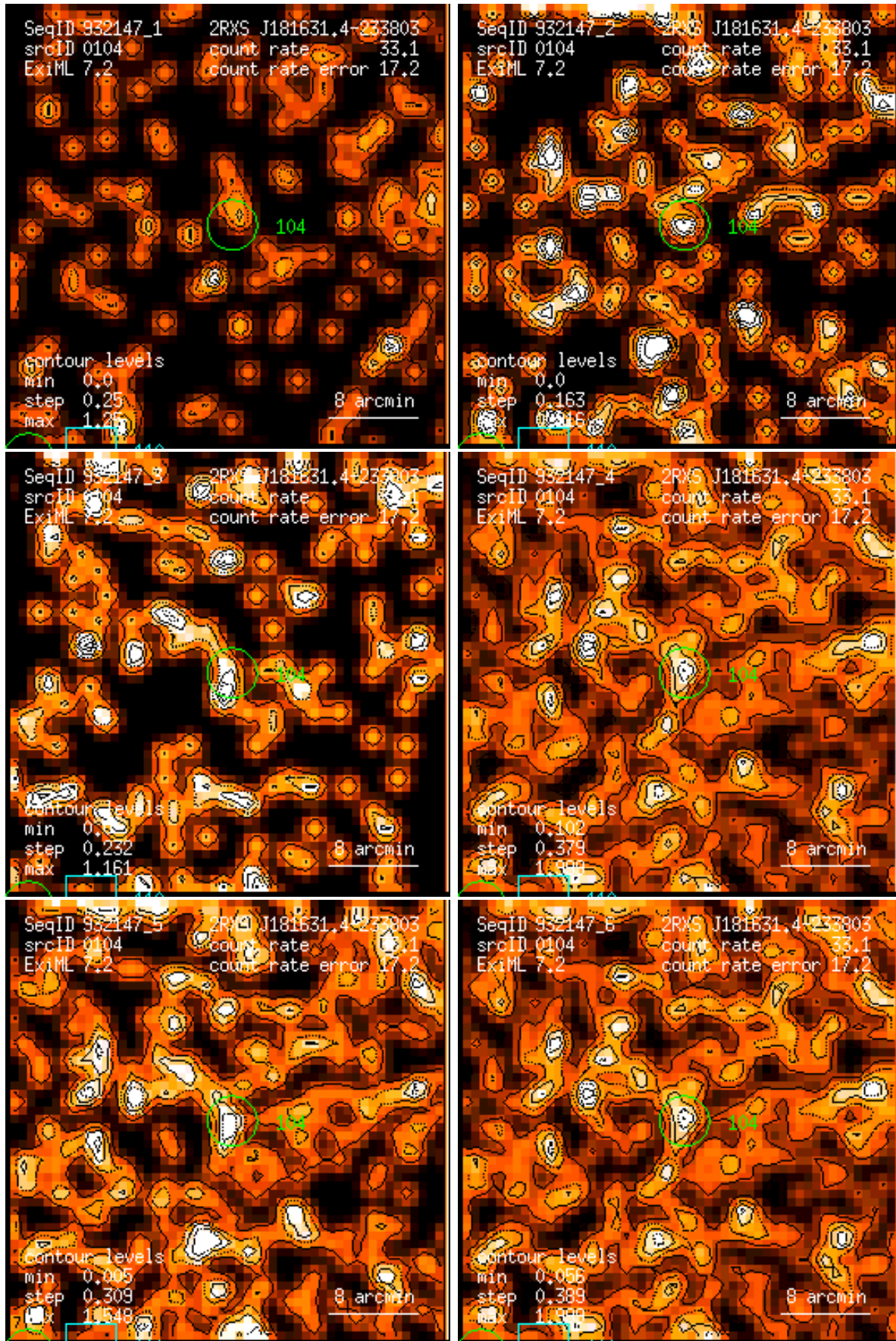
Figure 104: RASS 932147: detection 0104: band rate images, Gaussian filter: (1) PSPC channels 11 – 41, (2) 52 – 90, (3) 91 – 201, (4) 11 – 235, (5) 52 – 201, (6) 11 – 201. Broad band rates in counts/ks. Band rate contour levels in counts/ks/arcmin 2 .
