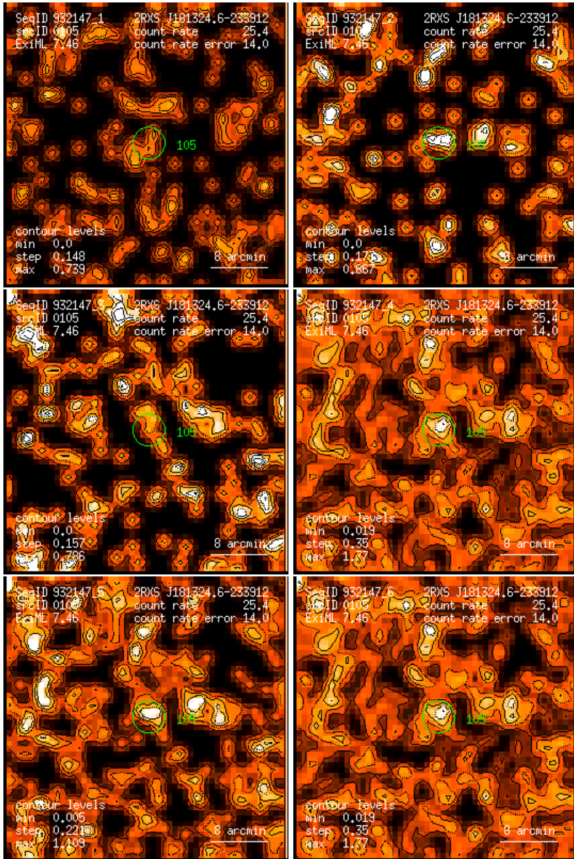
Figure 105: RASS 932147: detection 0105: band rate images, Gaussian filter: (1) PSPC channels 11 – 41, (2) 52 – 90, (3) 91 – 201, (4) 11 – 235, (5) 52 – 201, (6) 11 – 201. Broad band rates in counts/ks. Band rate contour levels in counts/ks/arcmin 2 .
