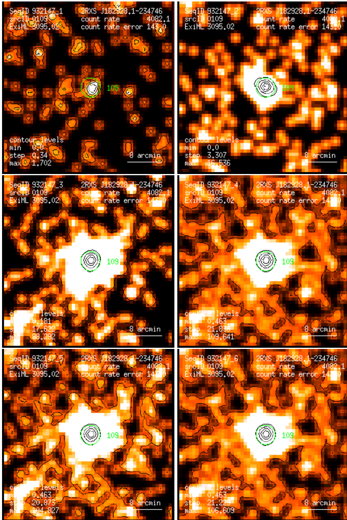
Figure 109: RASS 932147: detection 0109: band rate images, Gaussian filter: (1) PSPC channels 11 – 41, (2) 52 – 90, (3) 91 – 201, (4) 11 – 235, (5) 52 – 201, (6) 11 – 201. Broad band rates in counts/ks. Band rate contour levels in counts/ks/arcmin 2 .
