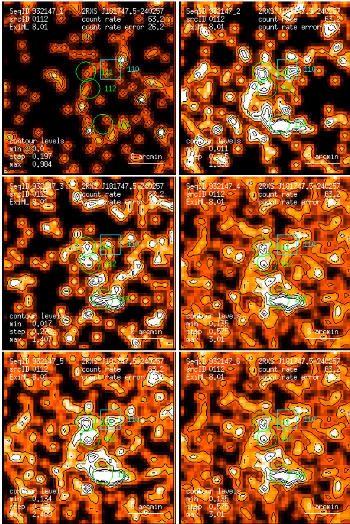
Figure 112: RASS 932147: detection 0112: band rate images, Gaussian filter: (1) PSPC channels 11 – 41, (2) 52 – 90, (3) 91 – 201, (4) 11 – 235, (5) 52 – 201, (6) 11 – 201. Broad band rates in counts/ks. Band rate contour levels in counts/ks/arcmin 2 .
