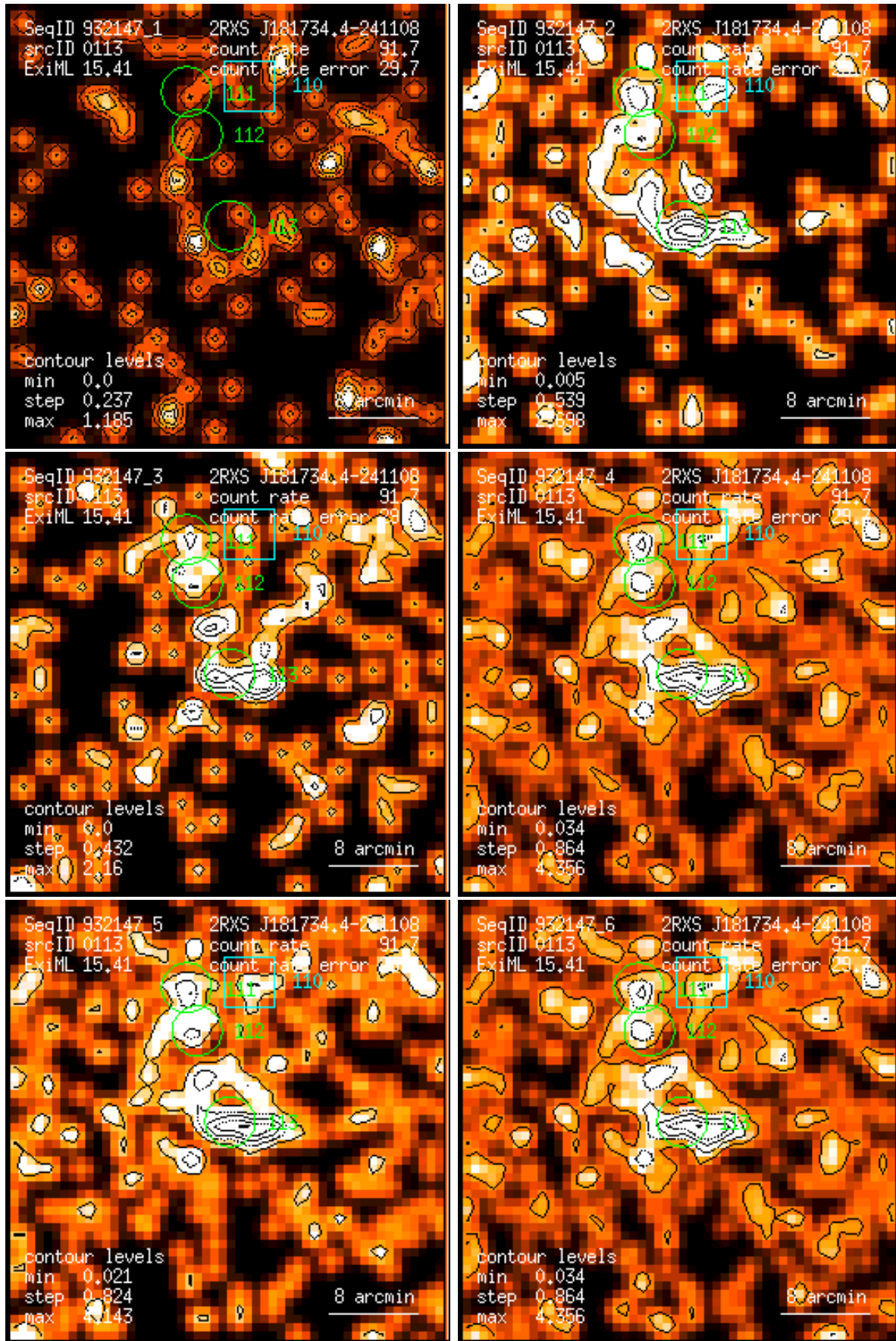
Figure 113: RASS 932147: detection 0113: band rate images, Gaussian filter: (1) PSPC channels 11 – 41, (2) 52 – 90, (3) 91 – 201, (4) 11 – 235, (5) 52 – 201, (6) 11 – 201. Broad band rates in counts/ks. Band rate contour levels in counts/ks/arcmin 2 .
