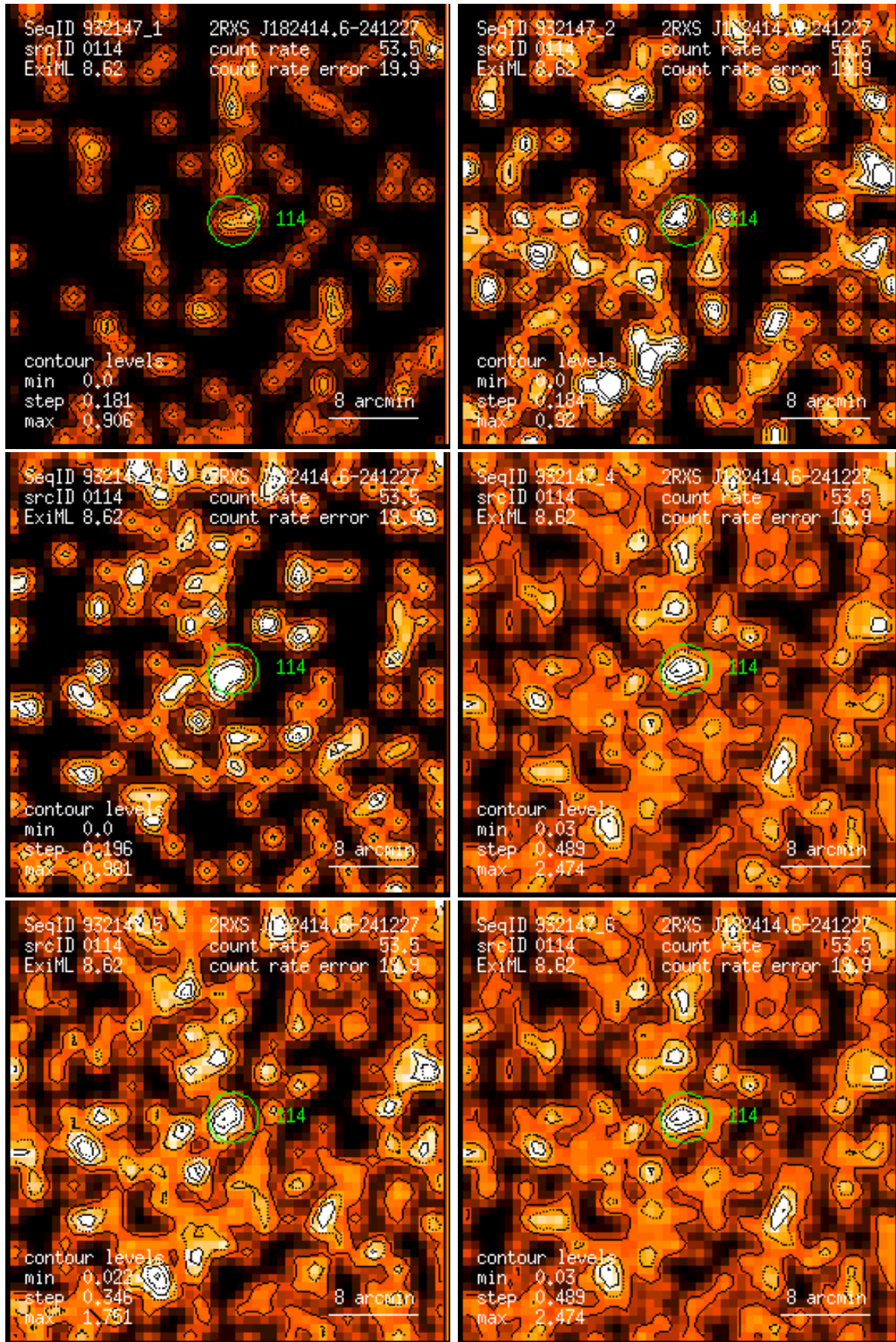
Figure 114: RASS 932147: detection 0114: band rate images, Gaussian filter: (1) PSPC channels 11 – 41, (2) 52 – 90, (3) 91 – 201, (4) 11 – 235, (5) 52 – 201, (6) 11 – 201. Broad band rates in counts/ks. Band rate contour levels in counts/ks/arcmin 2 .
