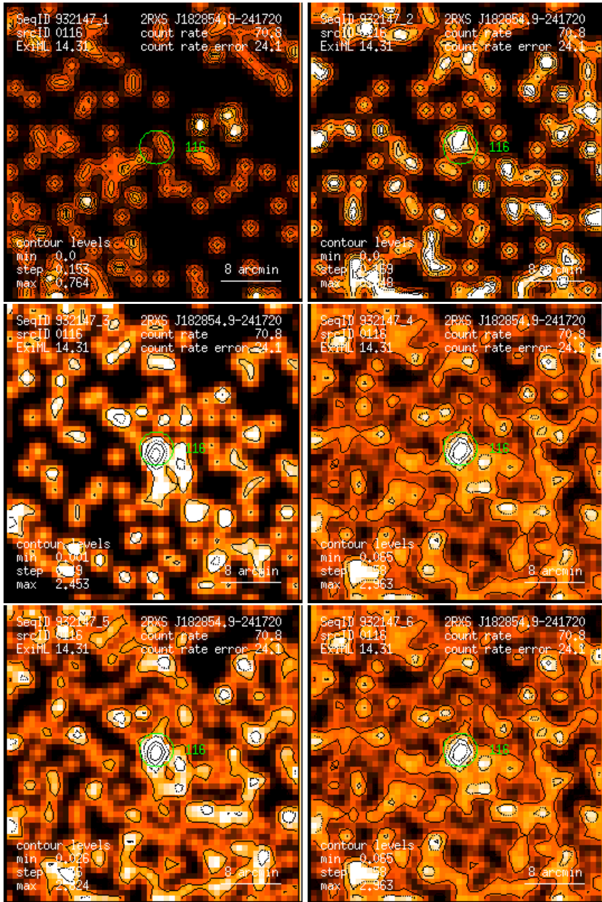
Figure 116: RASS 932147: detection 0116: band rate images, Gaussian filter: (1) PSPC channels 11 – 41, (2) 52 – 90, (3) 91 – 201, (4) 11 – 235, (5) 52 – 201, (6) 11 – 201. Broad band rates in counts/ks. Band rate contour levels in counts/ks/arcmin 2 .
