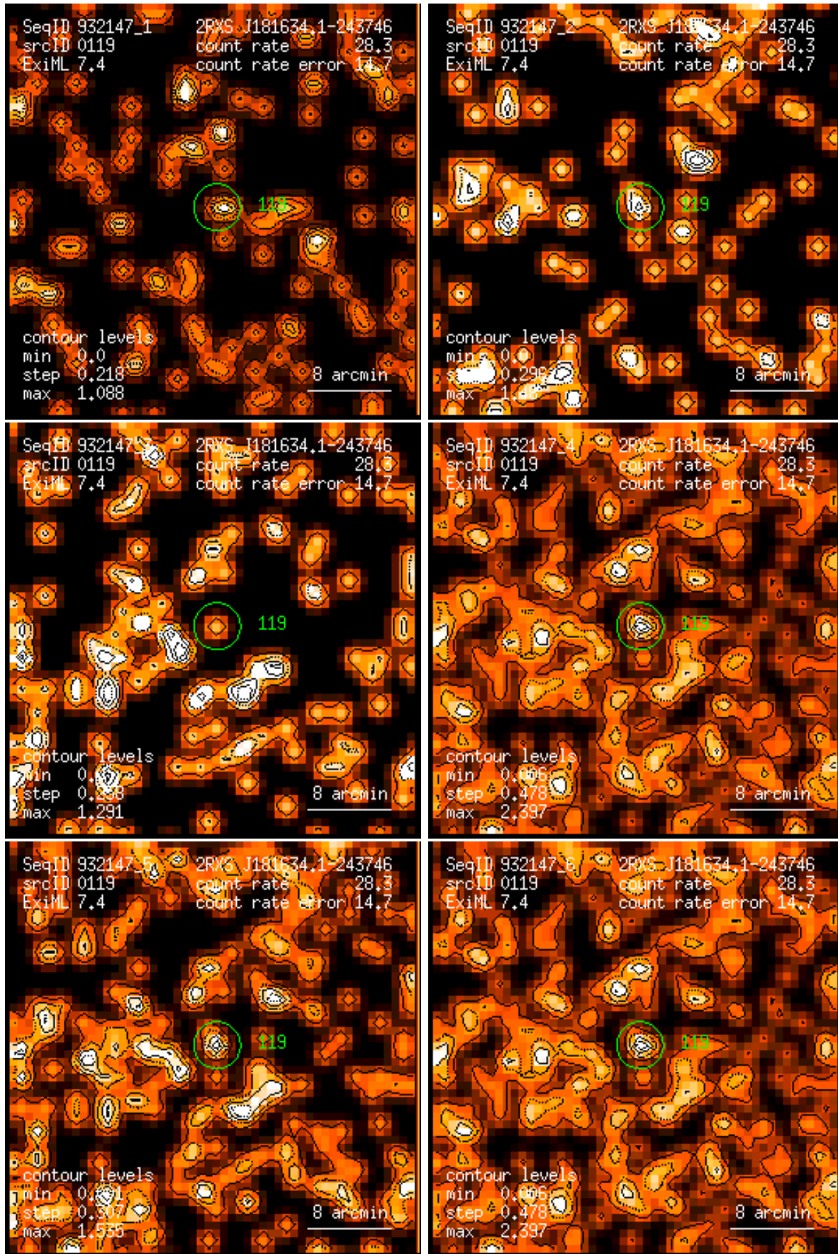
Figure 119: RASS 932147: detection 0119: band rate images, Gaussian filter: (1) PSPC channels 11 – 41, (2) 52 – 90, (3) 91 – 201, (4) 11 – 235, (5) 52 – 201, (6) 11 – 201. Broad band rates in counts/ks. Band rate contour levels in counts/ks/arcmin 2 .
