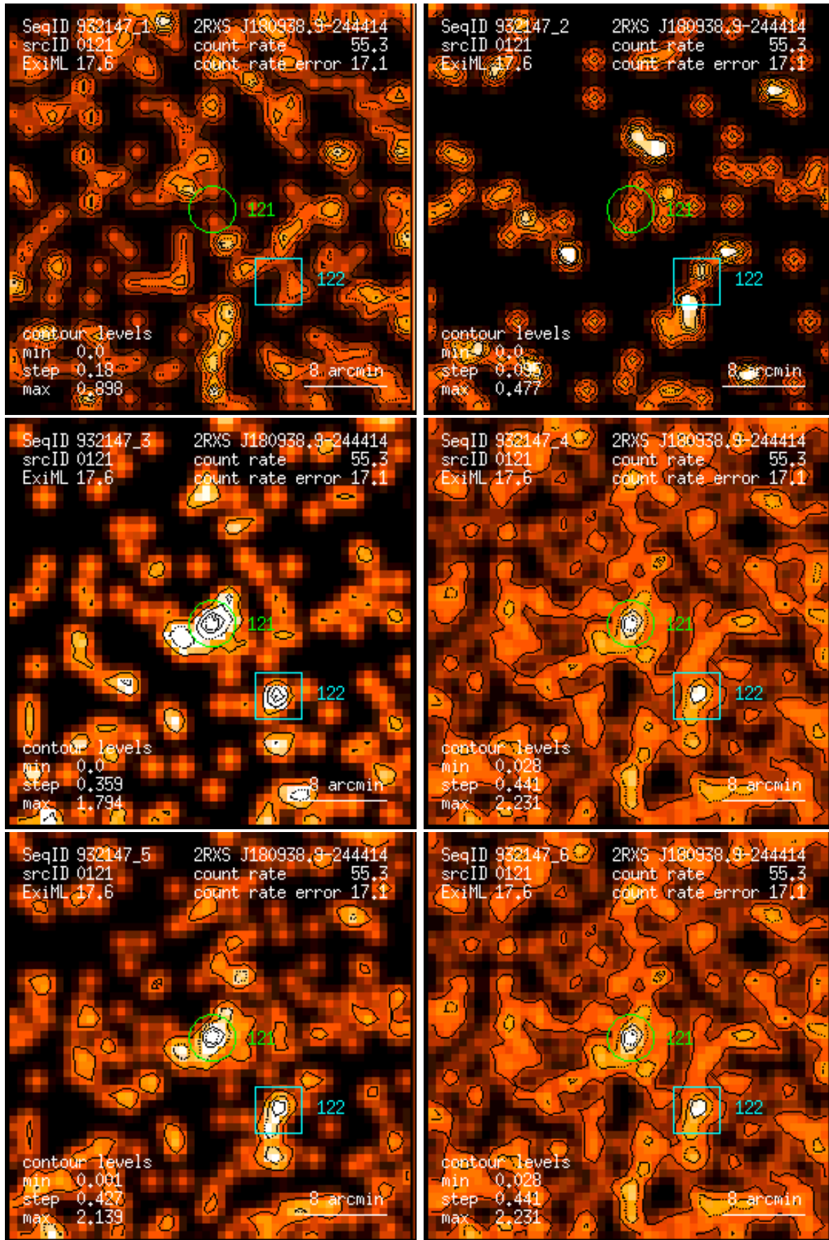
Figure 121: RASS 932147: detection 0121: band rate images, Gaussian filter: (1) PSPC channels 11 – 41, (2) 52 – 90, (3) 91 – 201, (4) 11 – 235, (5) 52 – 201, (6) 11 – 201. Broad band rates in counts/ks. Band rate contour levels in counts/ks/arcmin 2 .
