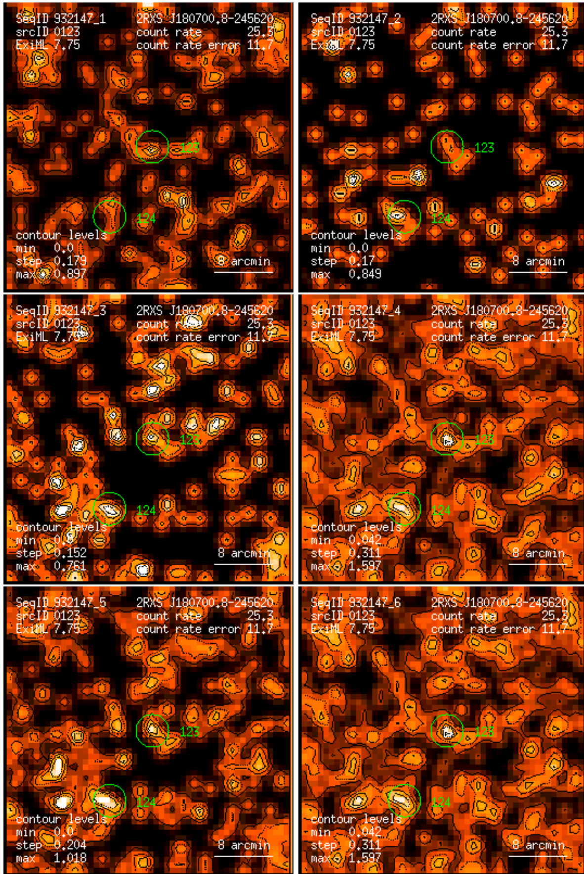
Figure 123: RASS 932147: detection 0123: band rate images, Gaussian filter: (1) PSPC channels 11 – 41, (2) 52 – 90, (3) 91 – 201, (4) 11 – 235, (5) 52 – 201, (6) 11 – 201. Broad band rates in counts/ks. Band rate contour levels in counts/ks/arcmin 2 .
