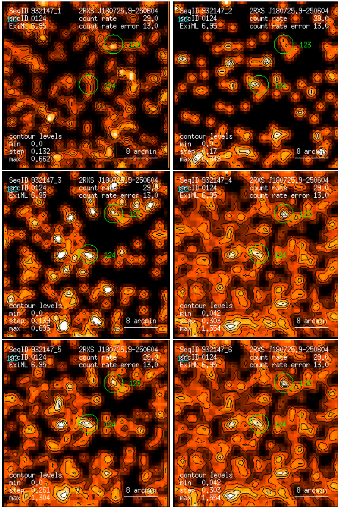
Figure 124: RASS 932147: detection 0124: band rate images, Gaussian filter: (1) PSPC channels 11 – 41, (2) 52 – 90, (3) 91 – 201, (4) 11 – 235, (5) 52 – 201, (6) 11 – 201. Broad band rates in counts/ks. Band rate contour levels in counts/ks/arcmin 2 .
