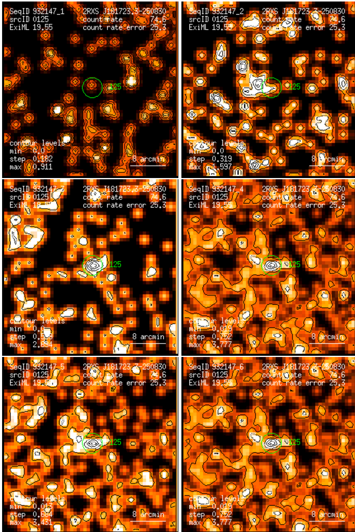
Figure 125: RASS 932147: detection 0125: band rate images, Gaussian filter: (1) PSPC channels 11 – 41, (2) 52 – 90, (3) 91 – 201, (4) 11 – 235, (5) 52 – 201, (6) 11 – 201. Broad band rates in counts/ks. Band rate contour levels in counts/ks/arcmin 2 .
