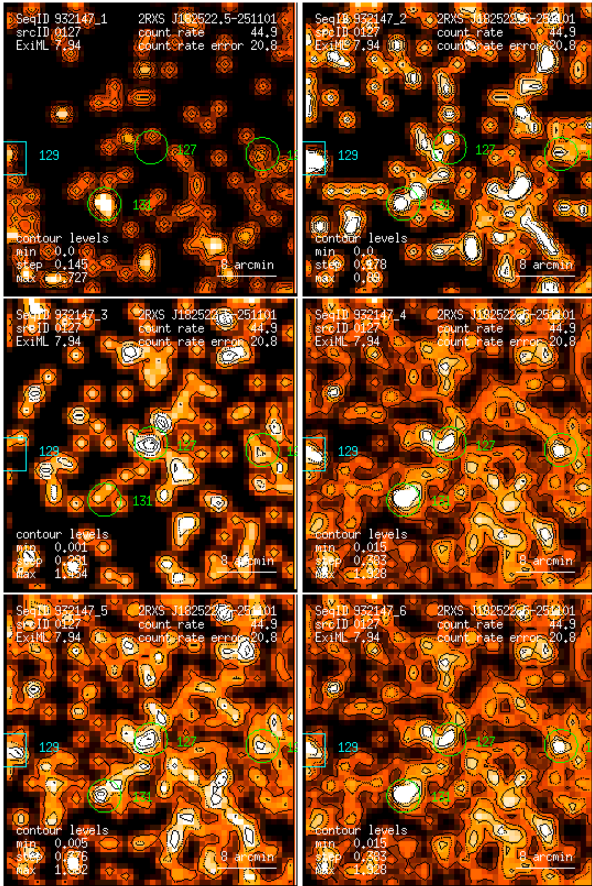
Figure 127: RASS 932147: detection 0127: band rate images, Gaussian filter: (1) PSPC channels 11 – 41, (2) 52 – 90, (3) 91 – 201, (4) 11 – 235, (5) 52 – 201, (6) 11 – 201. Broad band rates in counts/ks. Band rate contour levels in counts/ks/arcmin 2 .
